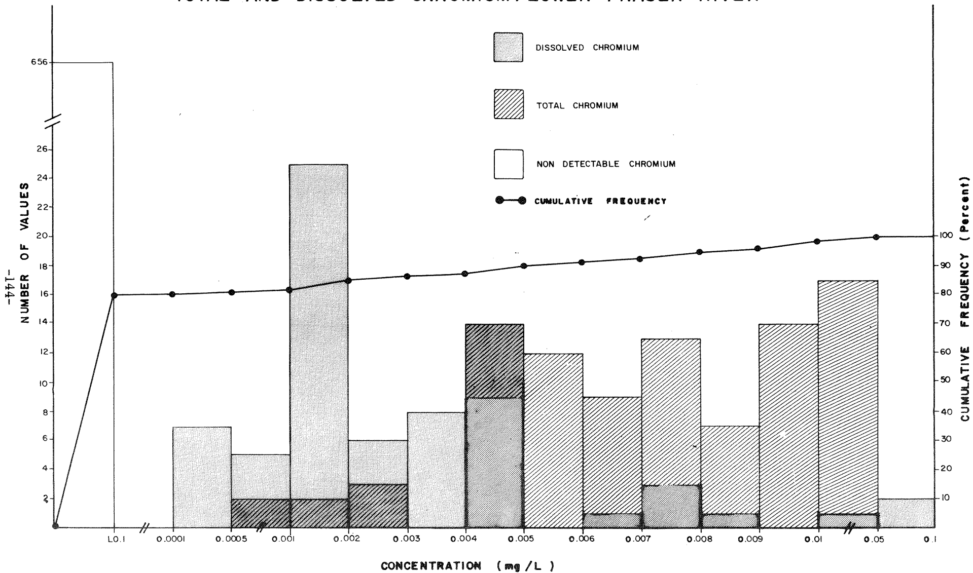
FIGURE 30 TOTAL AND DISSOLVED CHROMIUM; LOWER FRASER RIVER
