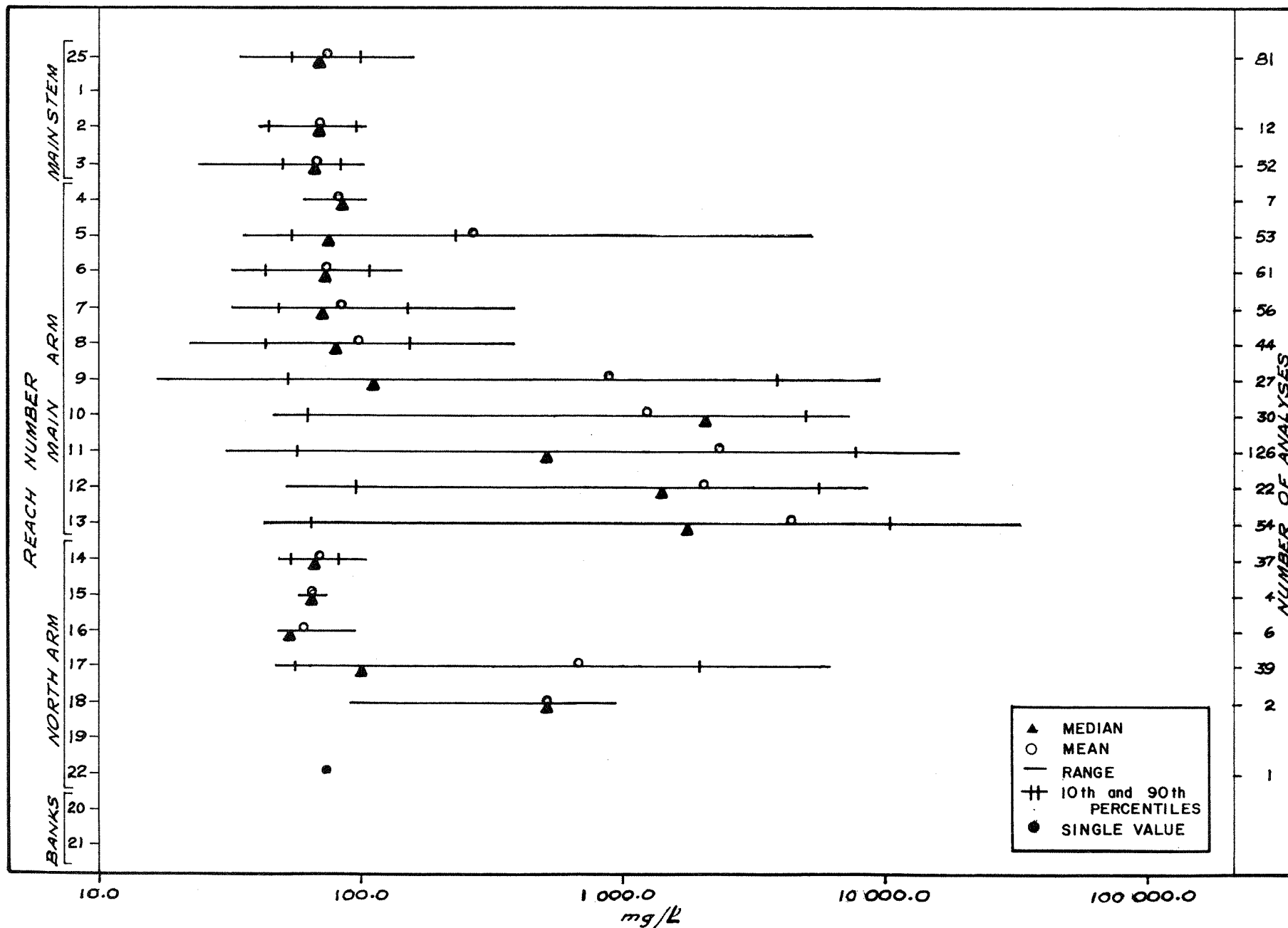
FIGURE II SUMMARY OF FILTERABLE RESIDUE DATA FOR THE INDIVIDUAL REACHES IN THE LOWER FRASER RIVER
