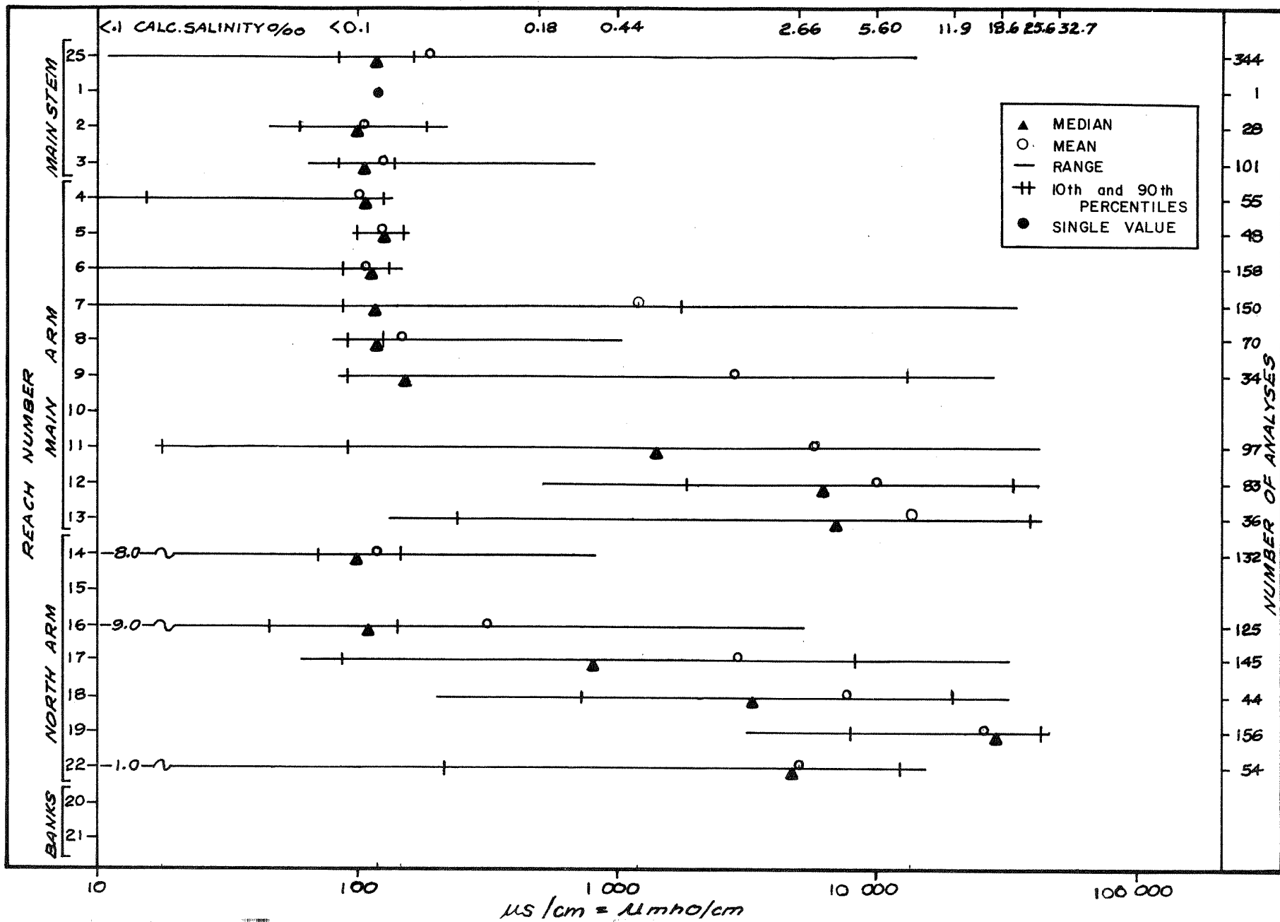
FIGURE 12 SUMMARY OF SPECIFIC CONDUCTIVITY DATA FOR THE INDIVIDUAL REACHES IN THE LOWER FRASER RIVER
