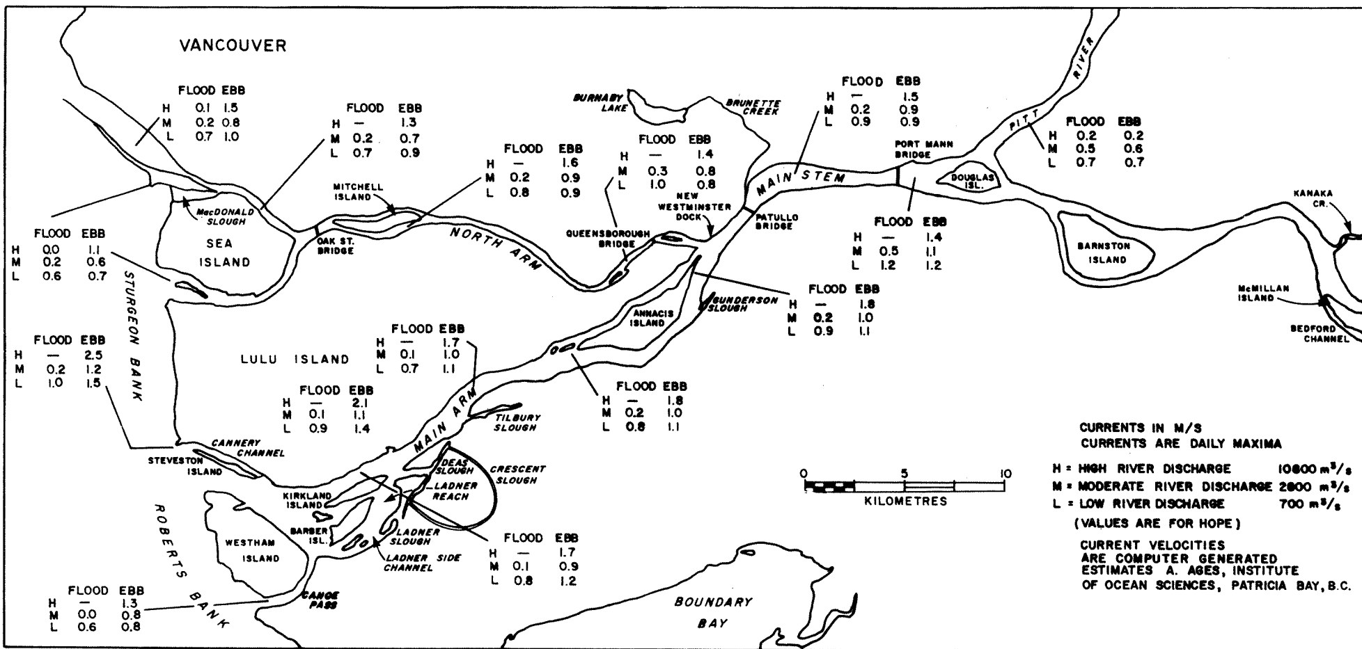
FIGURE 2 ESTIMATED DAILY MAXIMA OF CURRENTS FOR LOW, MODERATE AND HIGH RIVER DISCHARGES AT VARIOUS LOCATIONS IN THE LOWER FRASER RIVER
