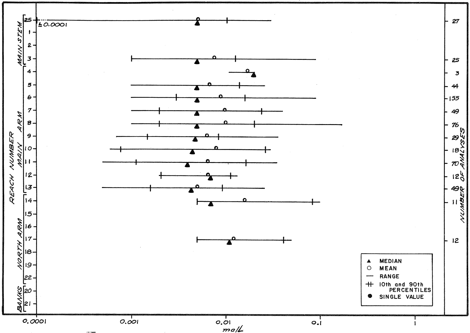
FIGURE 42 SUMMARY OF DISSOLVED ZINC DATA FOR THE INDIVIDUAL REACHES IN THE LOWER FRASER RIVER
