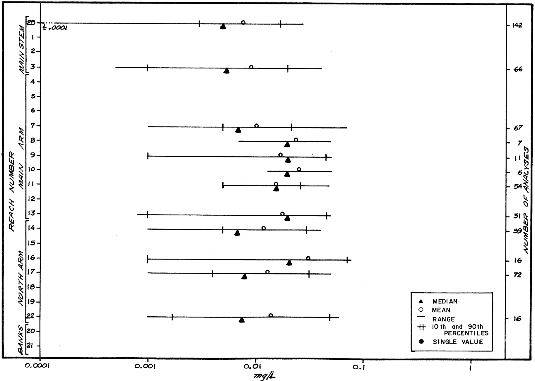
FIGURE 43 SUMMARY OF TOTAL ZINC DATA FOR THE INDIVIDUAL REACHES IN THE LOWER FRASER RIVER
