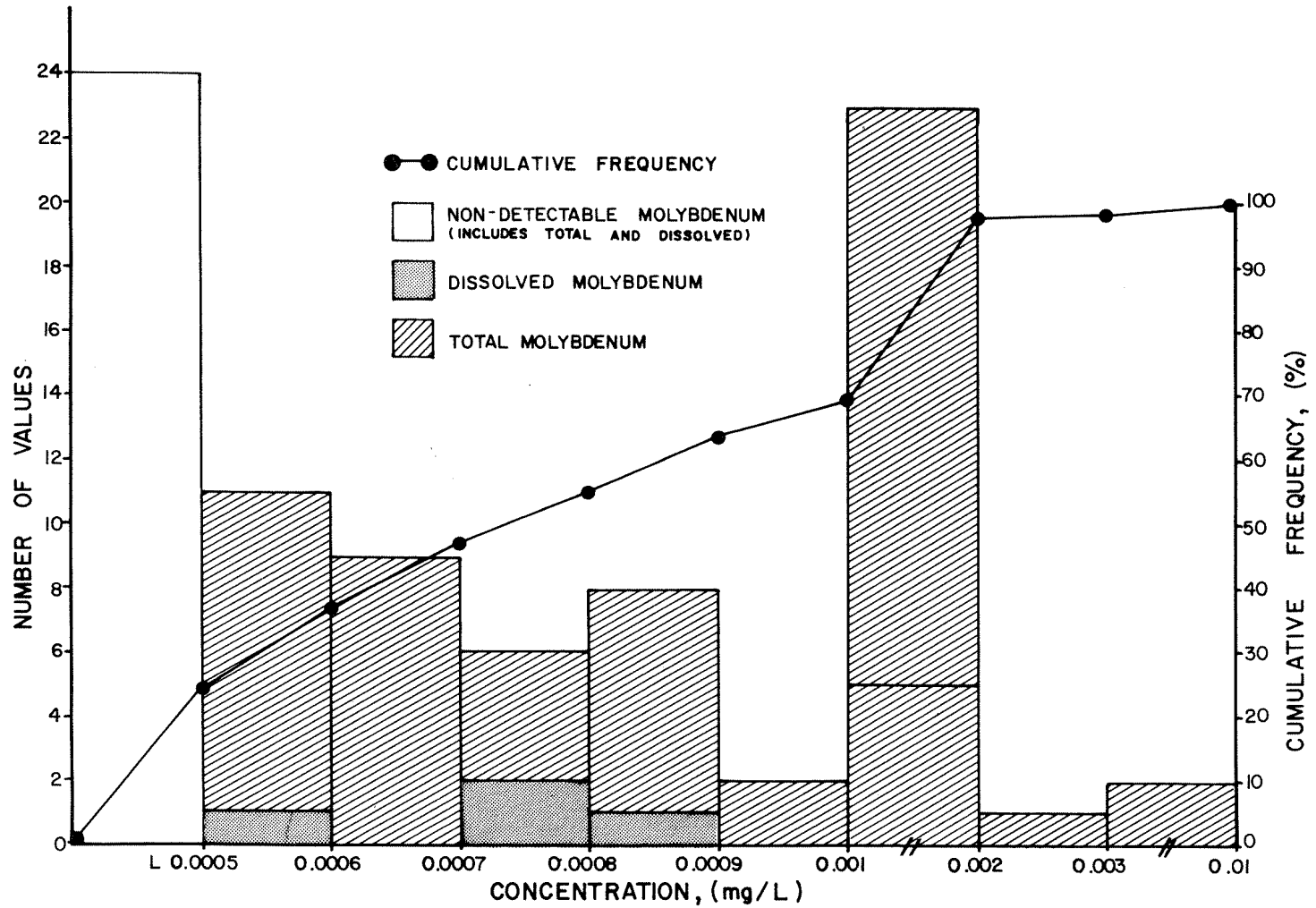
FIGURE 39 TOTAL AND DISSOLVED MOLYBDENUM; LOWER FRASER RIVER
