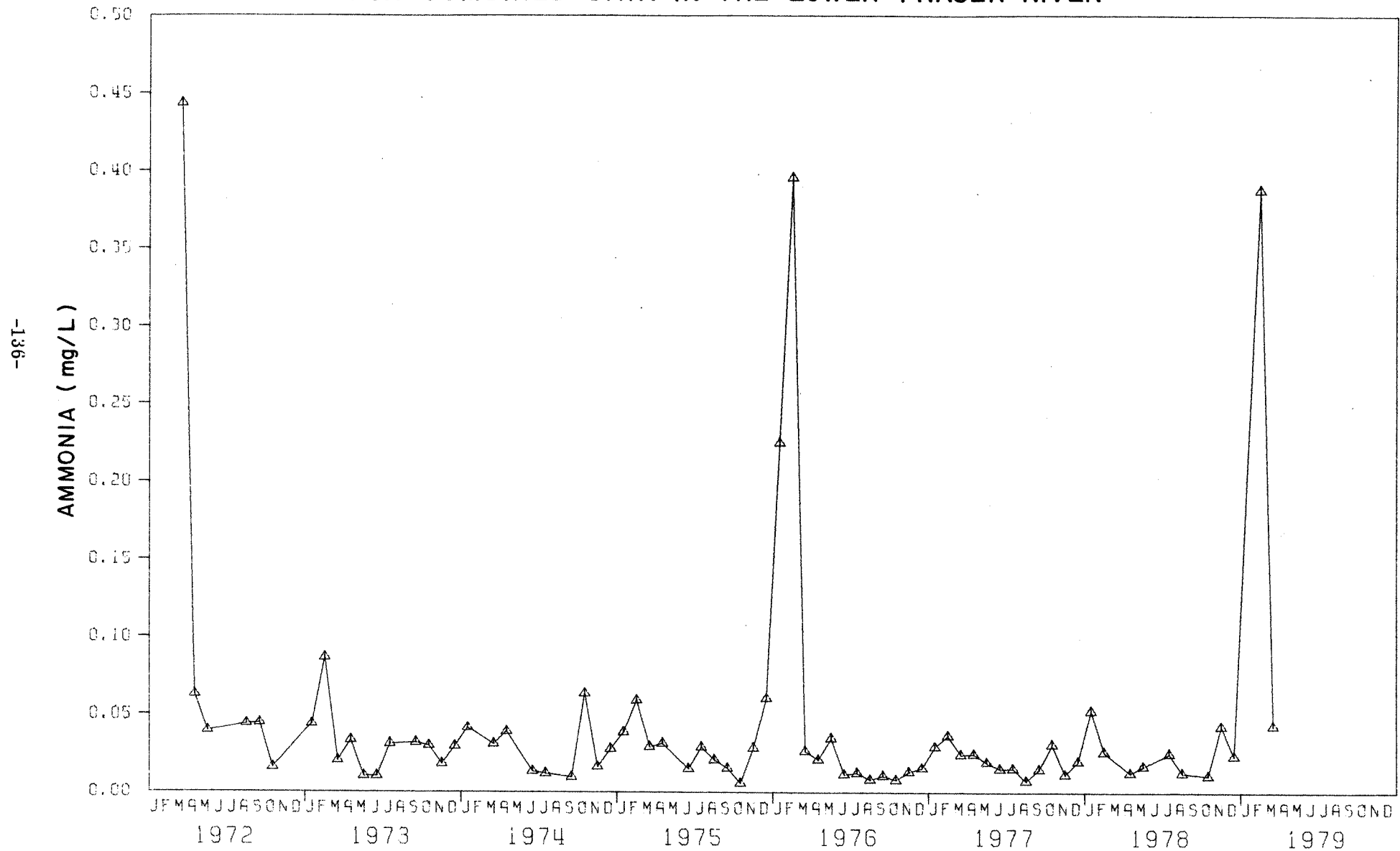
FIGURE 22 SEASONAL CHANGES (MONTHLY MEANS) IN AMMONIA FOR COMBINED DATA IN THE LOWER FRASER RIVER
