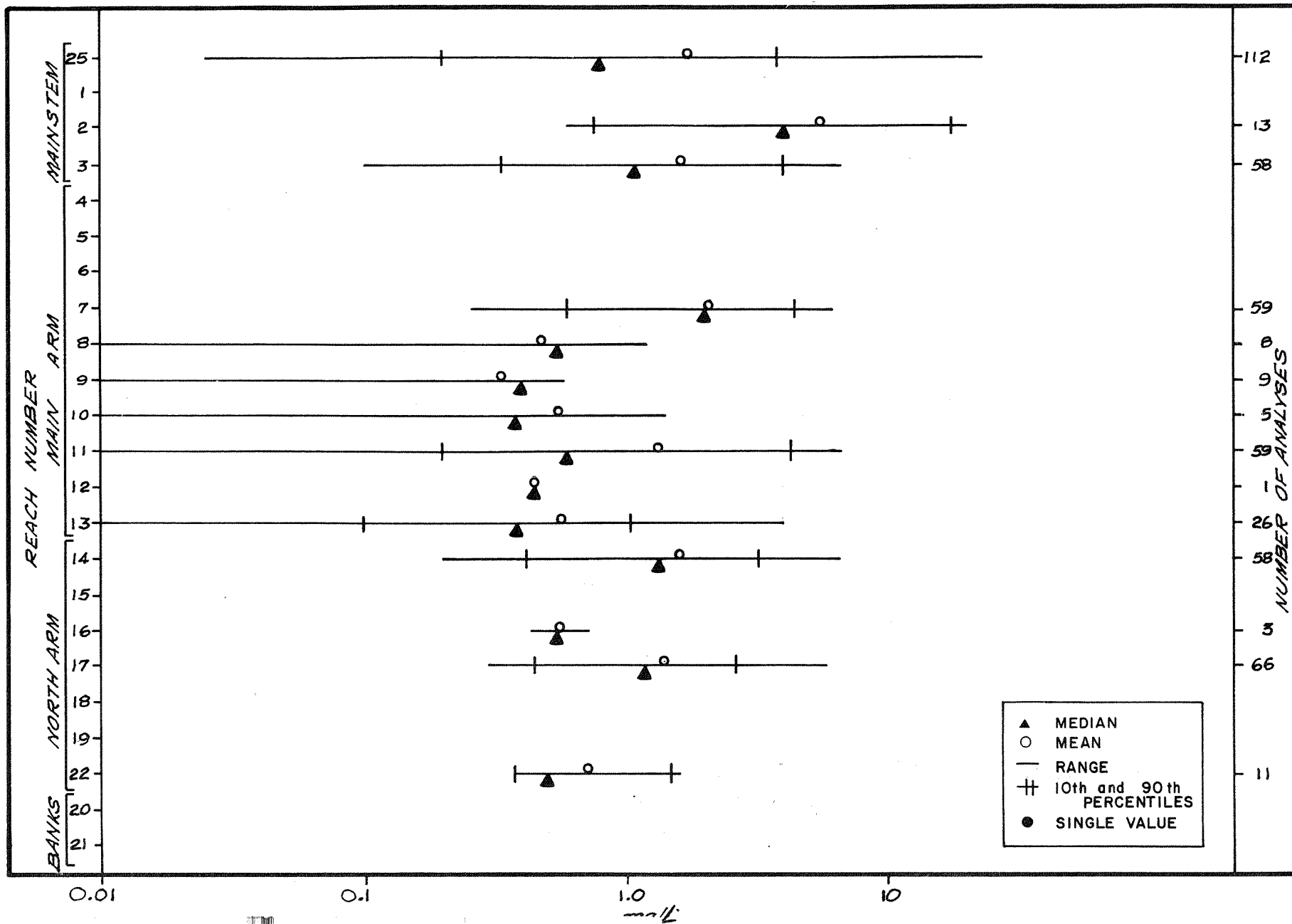
FIGURE 34 SUMMARY OF TOTAL IRON DATA FOR THE INDIVIDUAL REACHES IN THE LOWER FRASER RIVER
