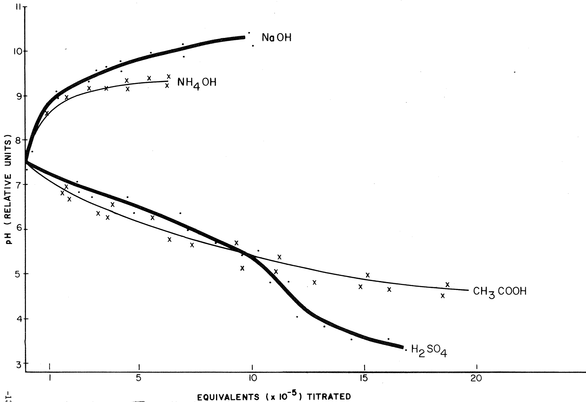
FIGURE 18 AVERAGE TITRATION CURVES OF THREE RIVER SAMPLES COLLECTED IN MAY AND JUNE, 1979 NEAR NEW WESTMINSTER (REACH 4)
