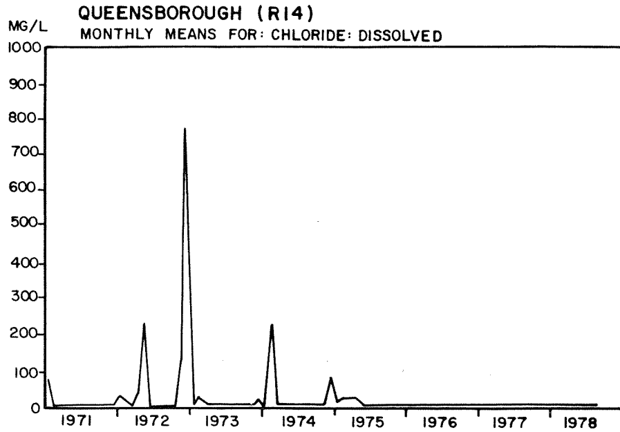
FIGURE 16 CHANGES IN MONTHLY CHLORIDE LEVELS: NORTH ARM
