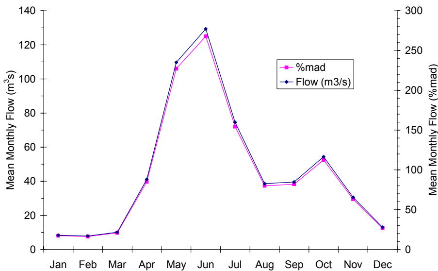
Figure 11. Annual hydrograph for the Kispiox River. Mean annual discharge = 45.1 m³/s (1963-99). Data are from the Water Survey of Canada monitoring station 08EB004.
