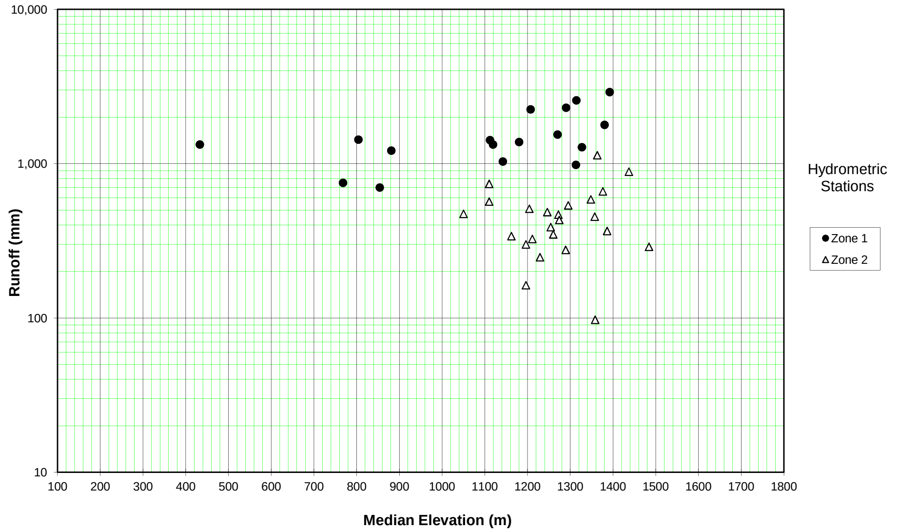
Figure 3 Normal Annual Runoff (page 1 of 2)
