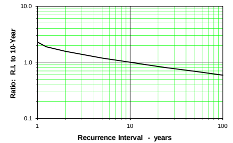
Annual 7-day Low Flow
