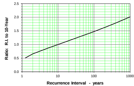
Instantaneous Peak Flow
