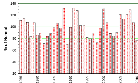
Annual Flow Variation
