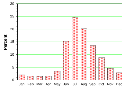
Monthly Flow Variation
