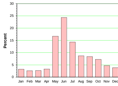
Monthly Flow Variation (Using Avg. Flow of 1989-2010)
