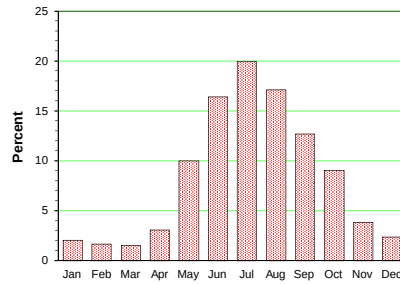
Monthly Flow Variation (Using Avg. Flow of 1981-1995/96)
