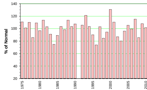
Annual Flow Variation
