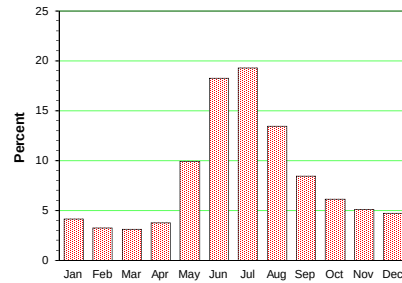
Monthly Flow Variation
