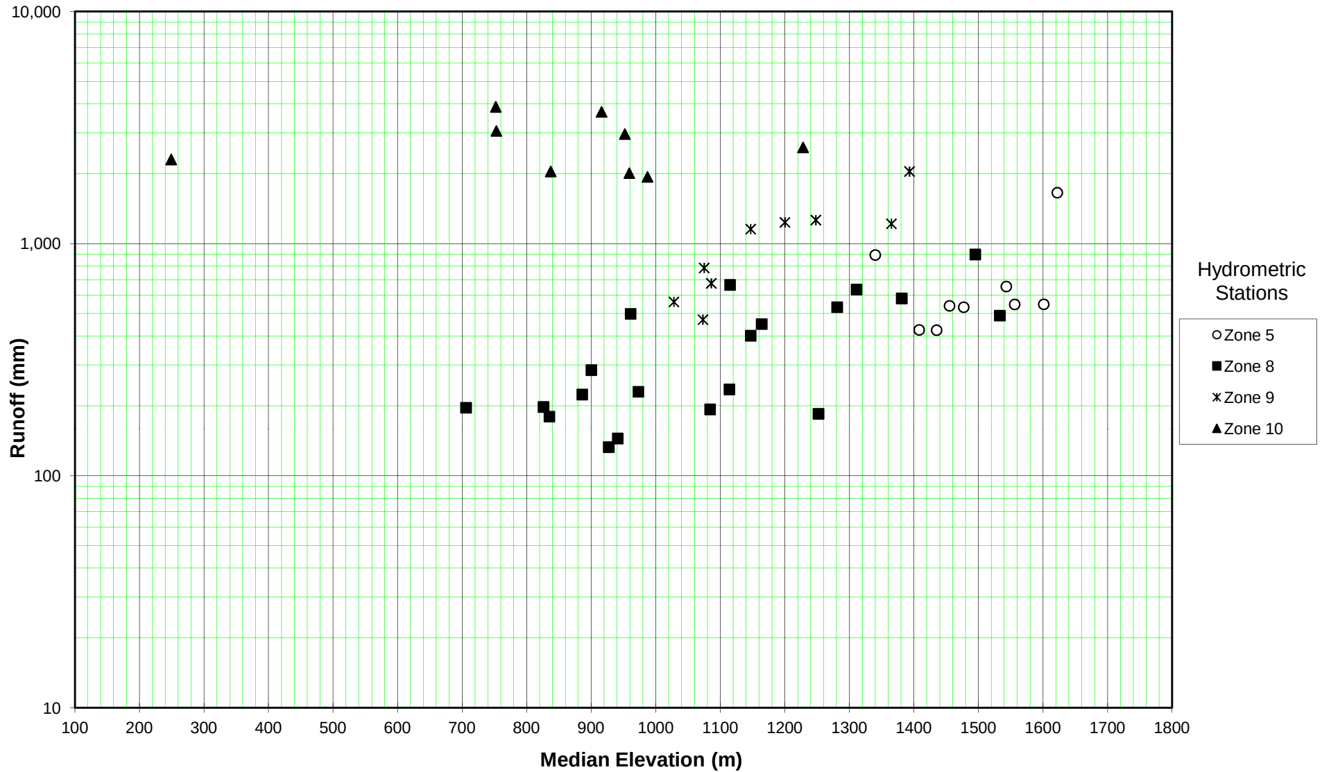
Figure 3 Normal Annual Runoff (page 2 of 2)
