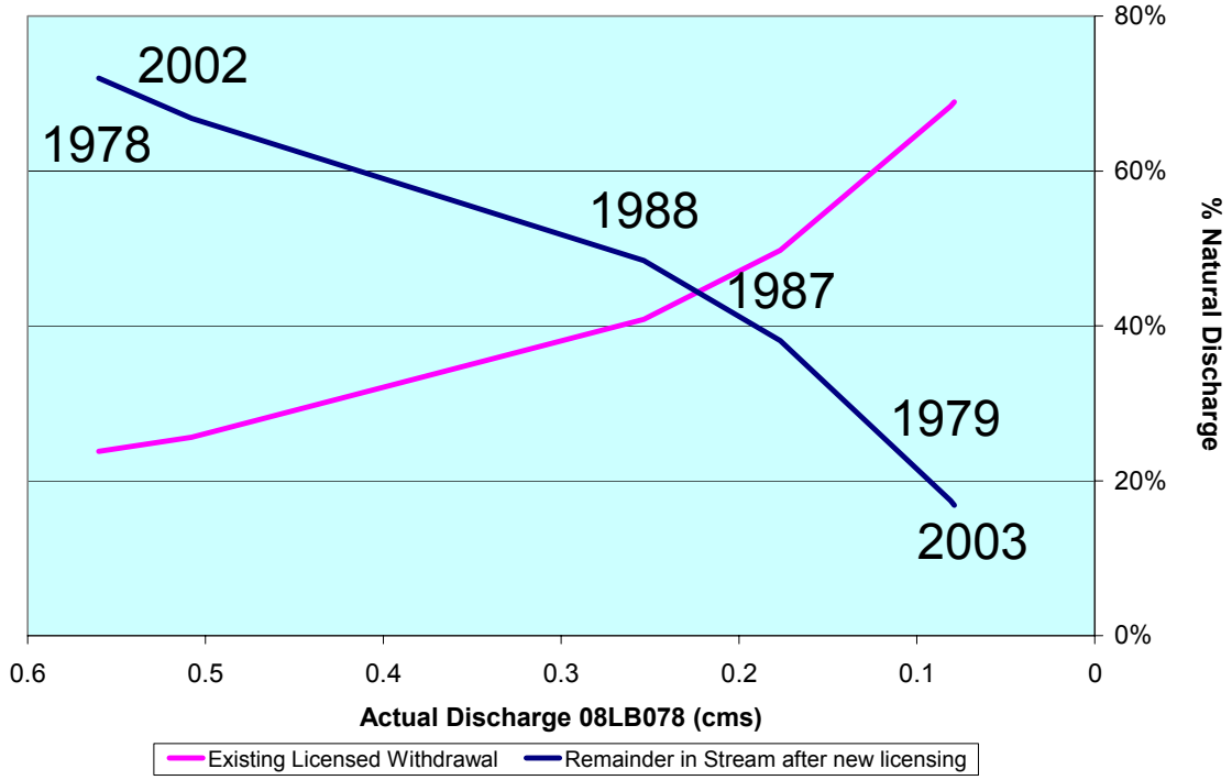
Lemieux Cr. Aug 8 Cutoff Scenario: In-stream/ off-stream Use Relationship
