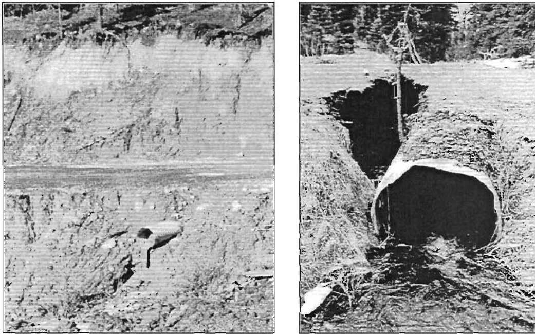
Figure 6. Improper installation or undersized culverts such as the one on a tributary to the Anahim Lake (left) or Horsefly drainage (right) can be significant sediment sources to fish bearing waters.
