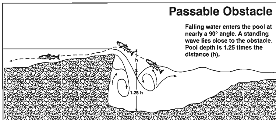
Figure 7. Optimal stream drop characteristics to allow fish passage (cited in Adams and Whyte 1990).
