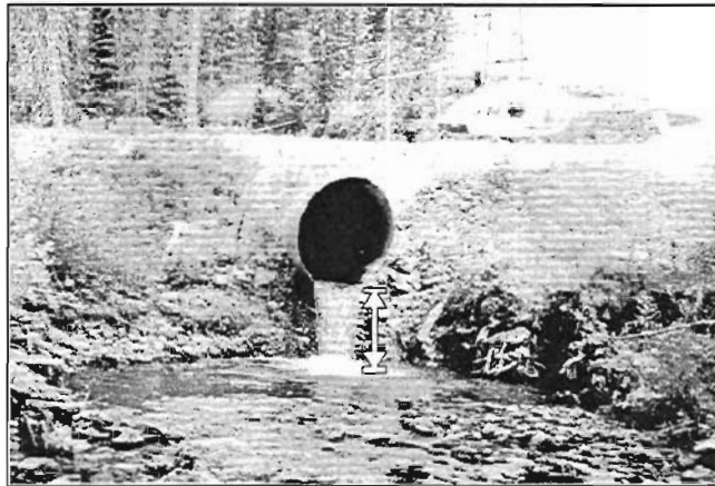
Figure 5. The culvert outfall drop is measured from the lip of the culvert to the water surface below. Photo at Foster Creek, Swift River watershed.
