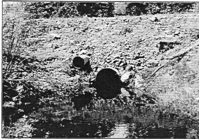
Figure 3. Stacked culverts in the Bradley Creek watershed. The smaller top culvert handles flows at extreme high flow periods.
