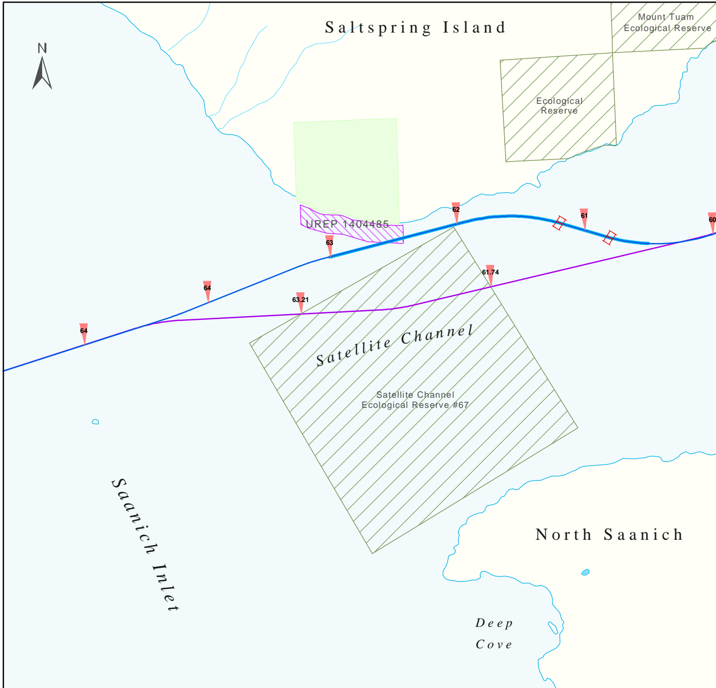
Figure 25 Satellite Channel - Pipeline Routing Options
