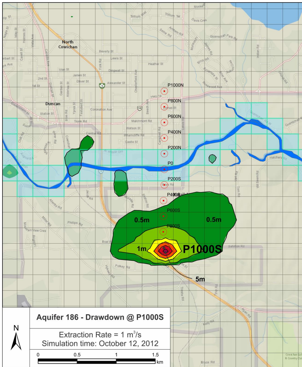
Figure 3.23. Drawdown during distance - sensitivity test. Pumping occurring at P1000S location ( 1 \text{ m}^3/\text{s} ).
