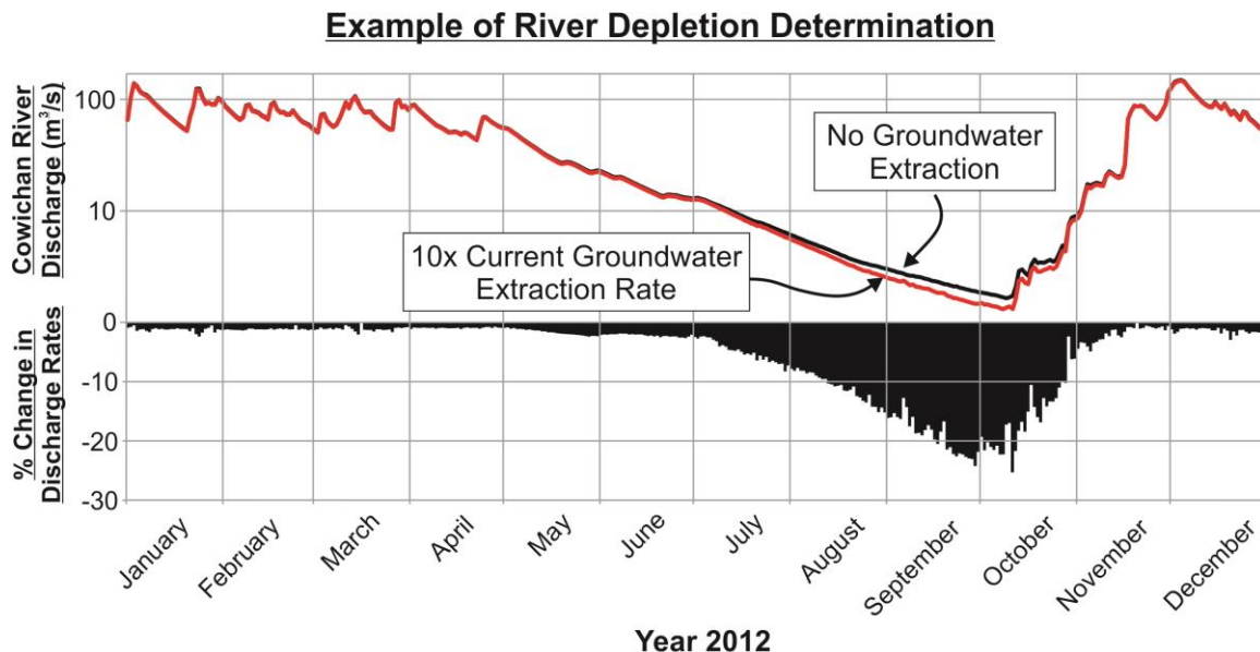
Figure 3.18. Example of the method used for estimating river depletion from pumping an individual well. Shown are the results for RN4 (Marine Harvest Hatchery) in 2012 at 10X current extraction rate.
