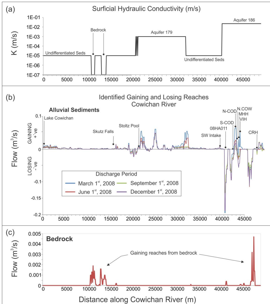
Figure 3.7. The relationship between (a) aquifer hydraulic conductivity, (b) seasonal variations to GW-SW interactions, and (c) the contribution of bedrock aquifers.
