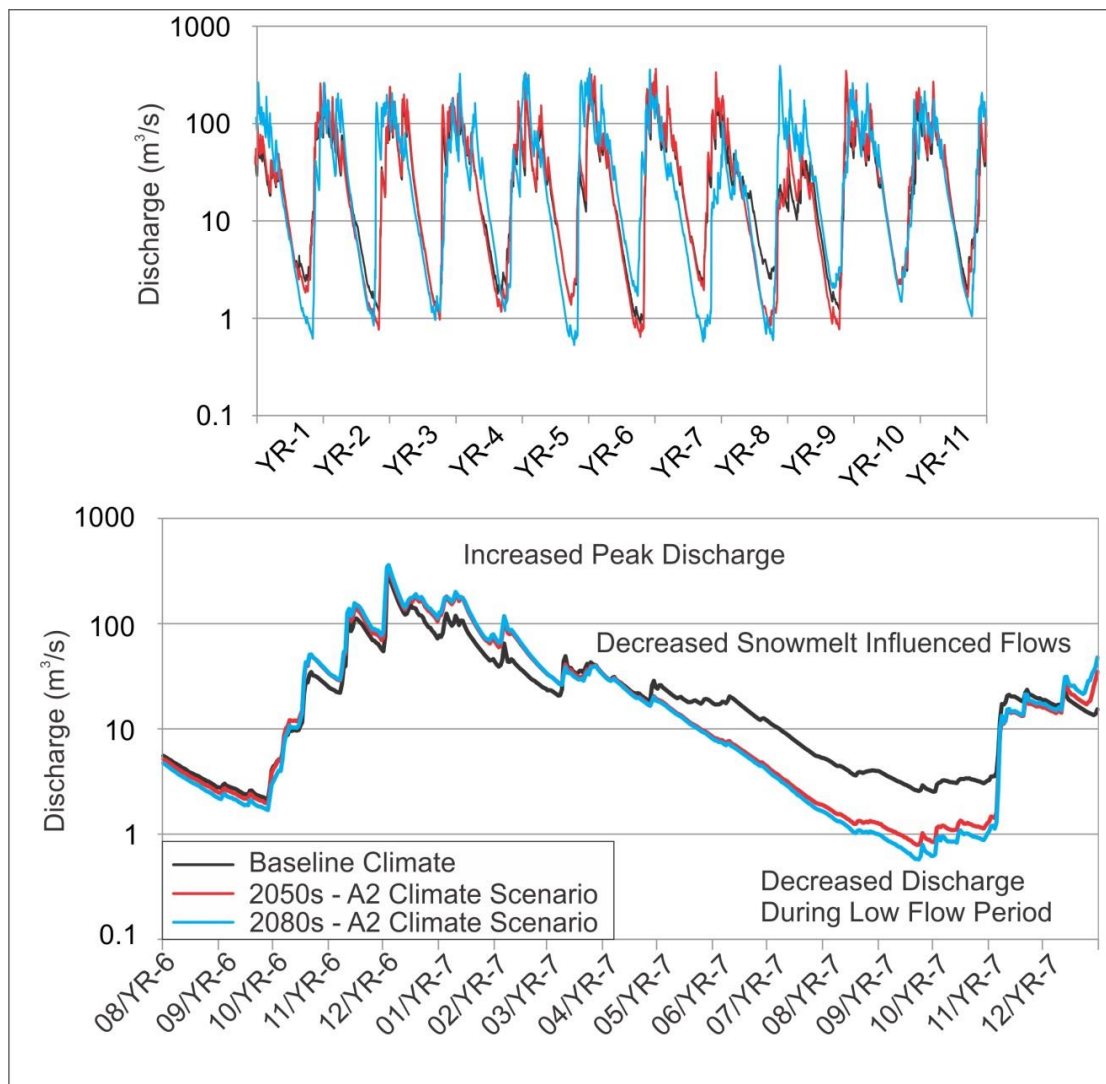
Figure 3.33. Simulated Cowichan River flows under baseline and climate change conditions (from Foster and Allen 2015).
