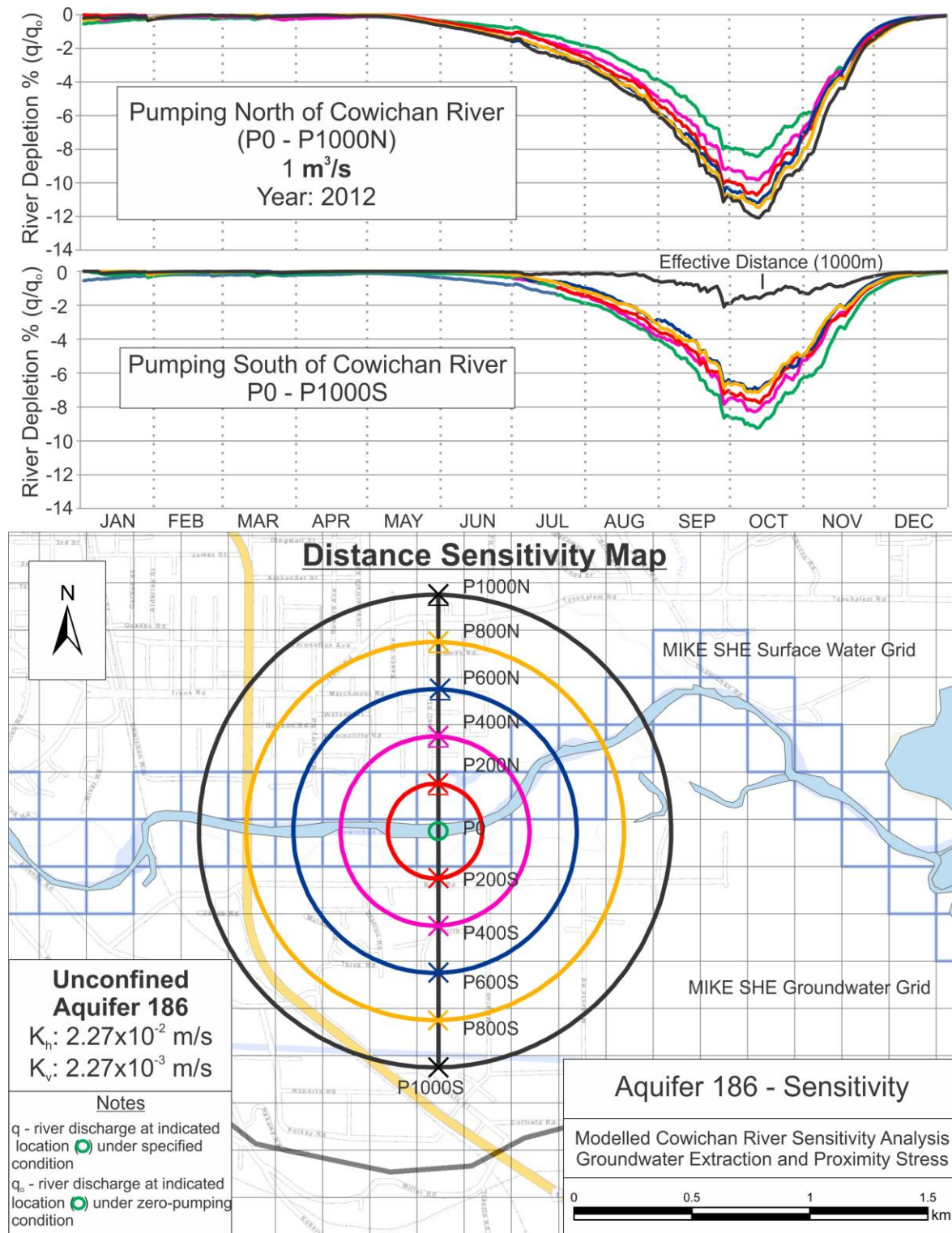
Figure 3.20. Modelled Cowichan River distance - sensitivity assessment for Aquifer 186 (1 m³/s pumping rate).
