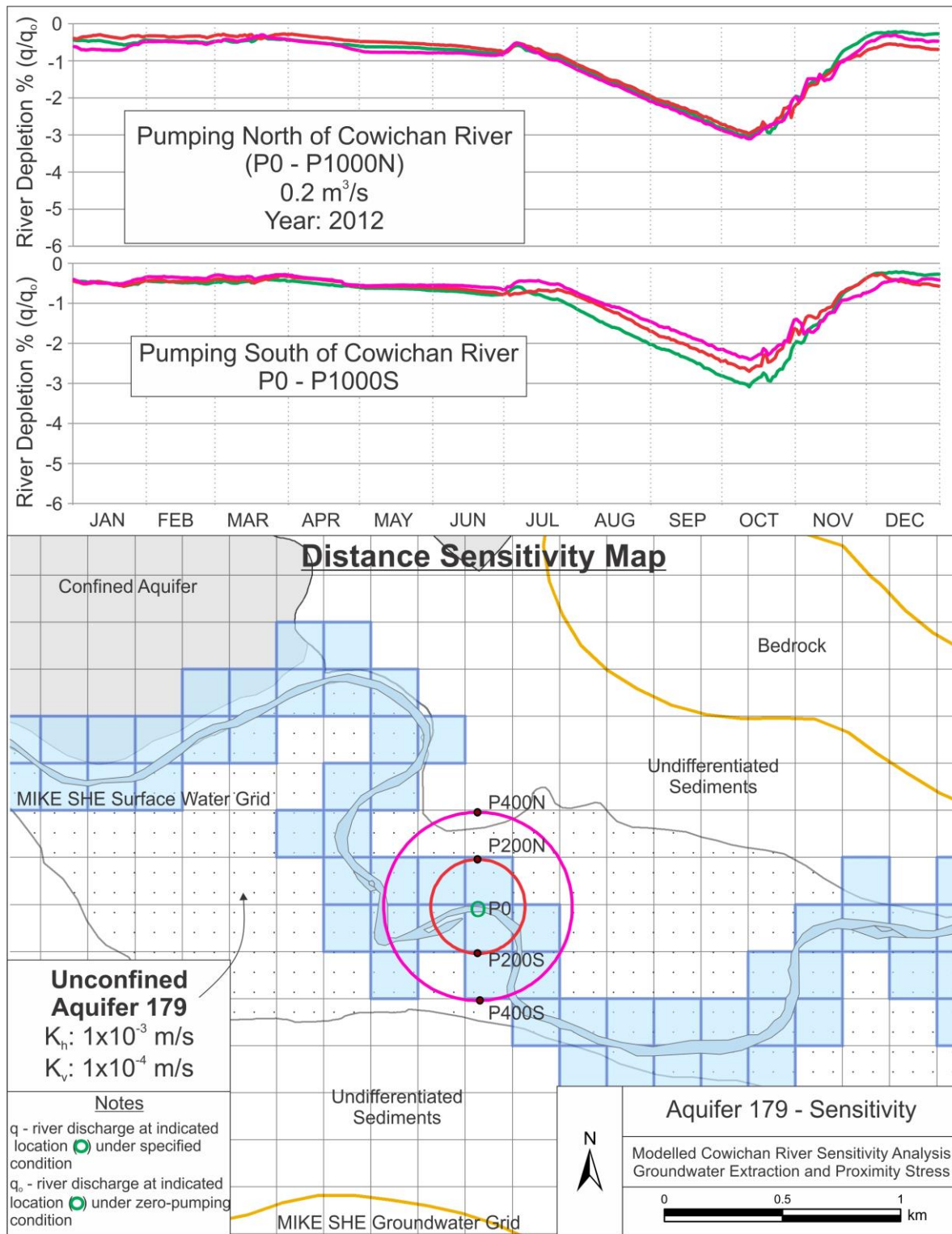
Figure A2.1. Modelled Cowichan River distance - sensitivity assessment for Aquifer 179 (0.2 m³/s pumping rate).
