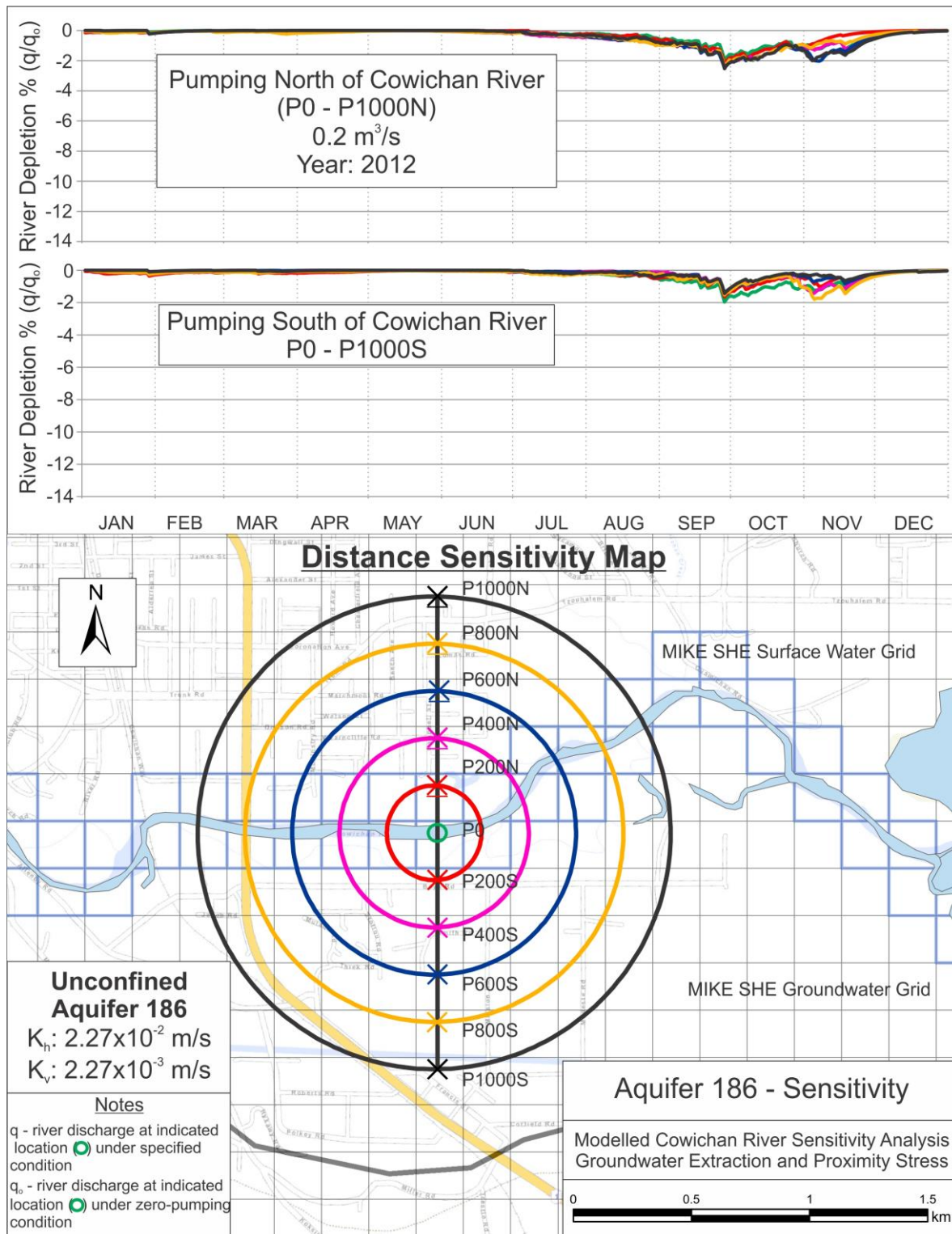
Figure 3.24. Modelled Cowichan River distance - sensitivity assessment for Aquifer 186 (0.2 m³/s pumping rate).
