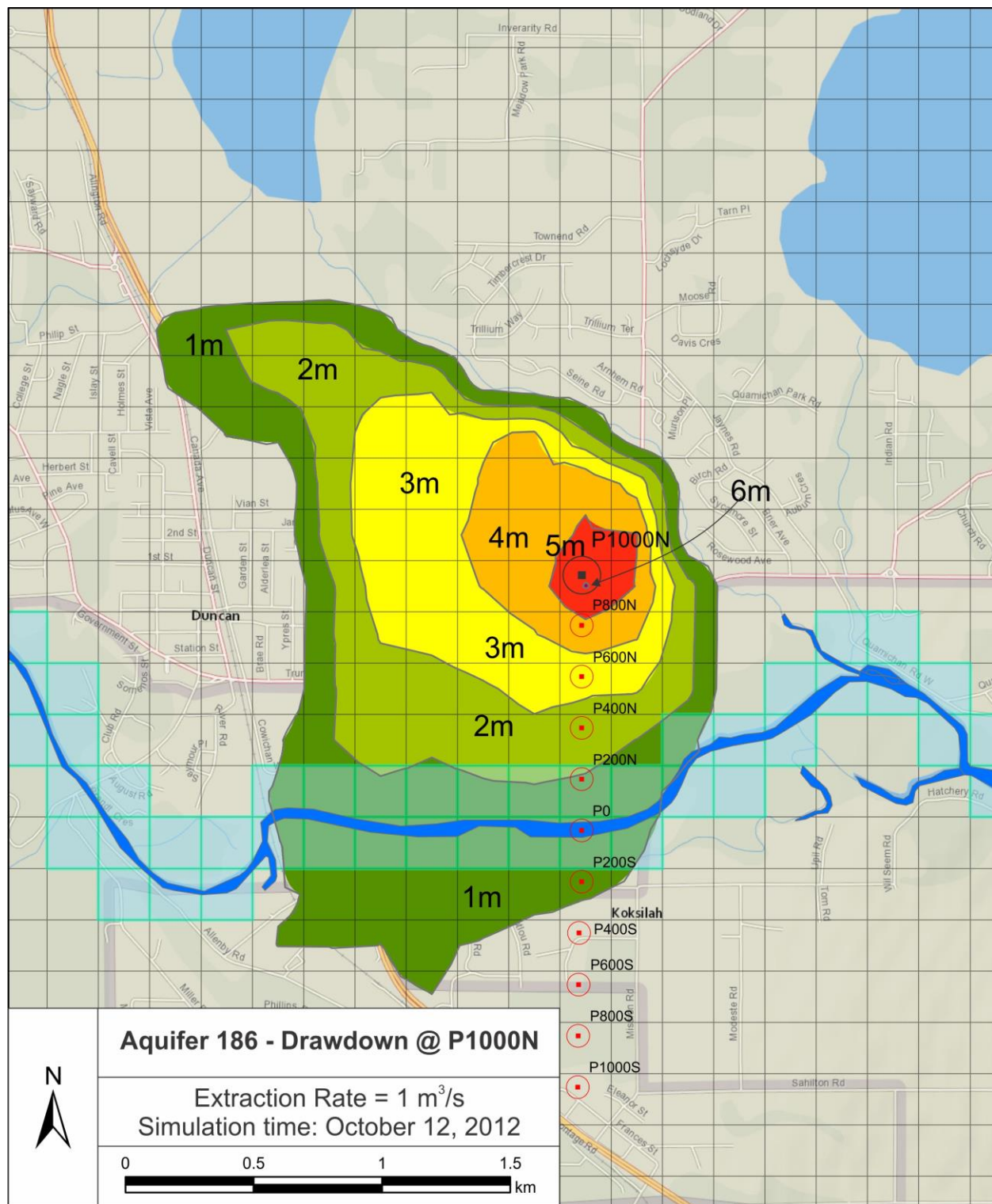
Figure 3.22. Drawdown during distance - sensitivity test. Pumping occurring at P1000N location ( 1 \text{ m}^3/\text{s} ).
