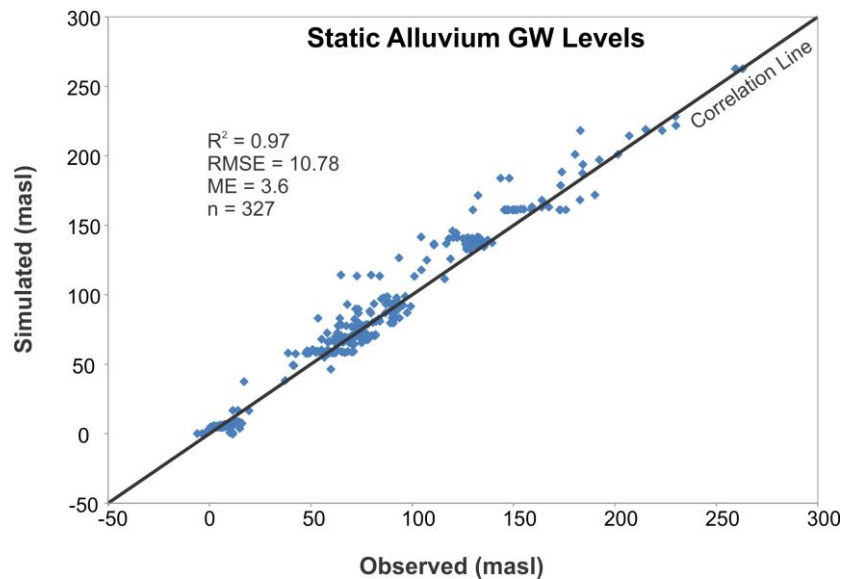
Figure 3.1. Simulated mean annual (2007) alluvial GW elevations verses observed static GW elevations in the alluvium from the BC WELLS database.
