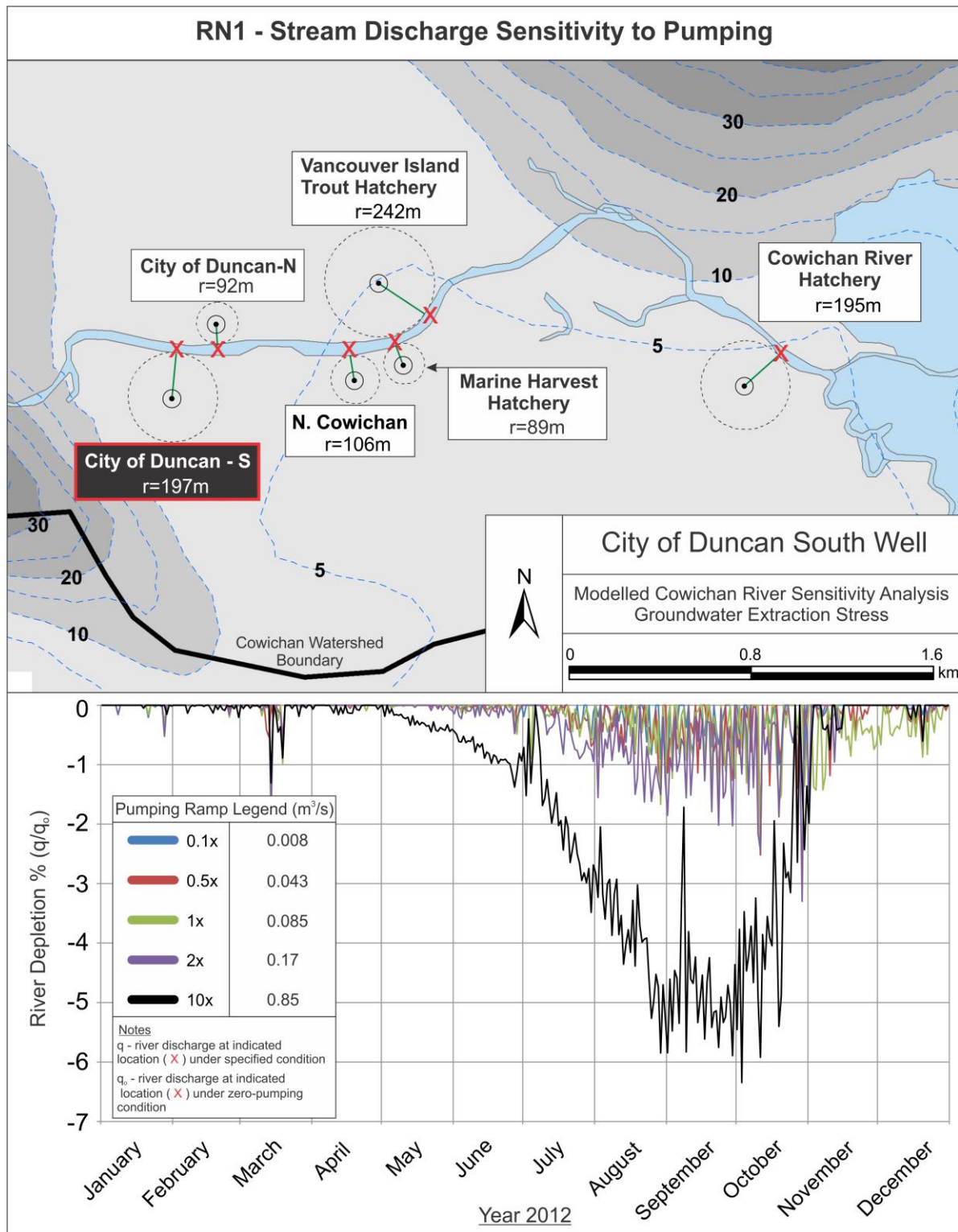
Figure A1.1. Cowichan River depletion assessment - variable pumping rates for the City of Duncan S well.
