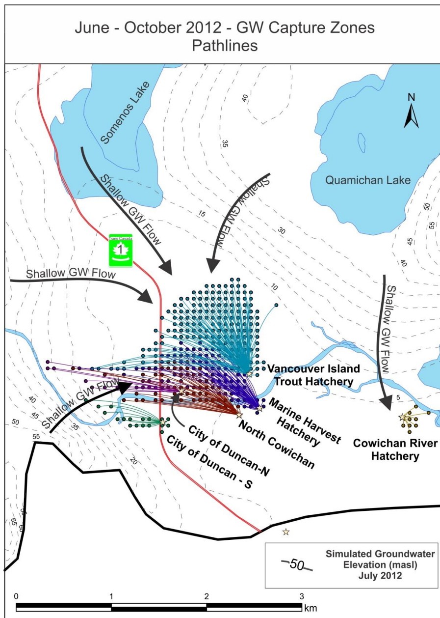
Figure 3.13. Summer low flow season transient capture zone analysis results for the major GW extraction users within the lower valley. Shown are the particle pathlines within the shallow aquifer materials.
