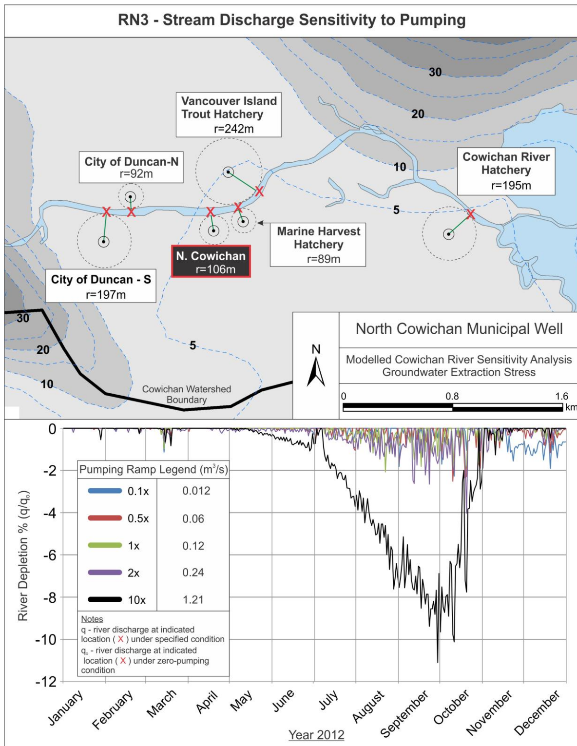
Figure A1.3. Cowichan River depletion assessment - variable pumping rates for the municipality of North Cowichan well.
