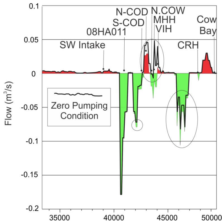
Figure 3.10. Simulated influence of GW pumping on GW/SW interactions (from Foster and Allen 2015).
