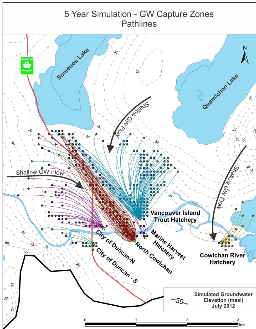
Figure 3.14. 5-year transient groundwater capture zone analysis (2008-2012). Shown are the particle pathlines within the shallow aquifer materials.
