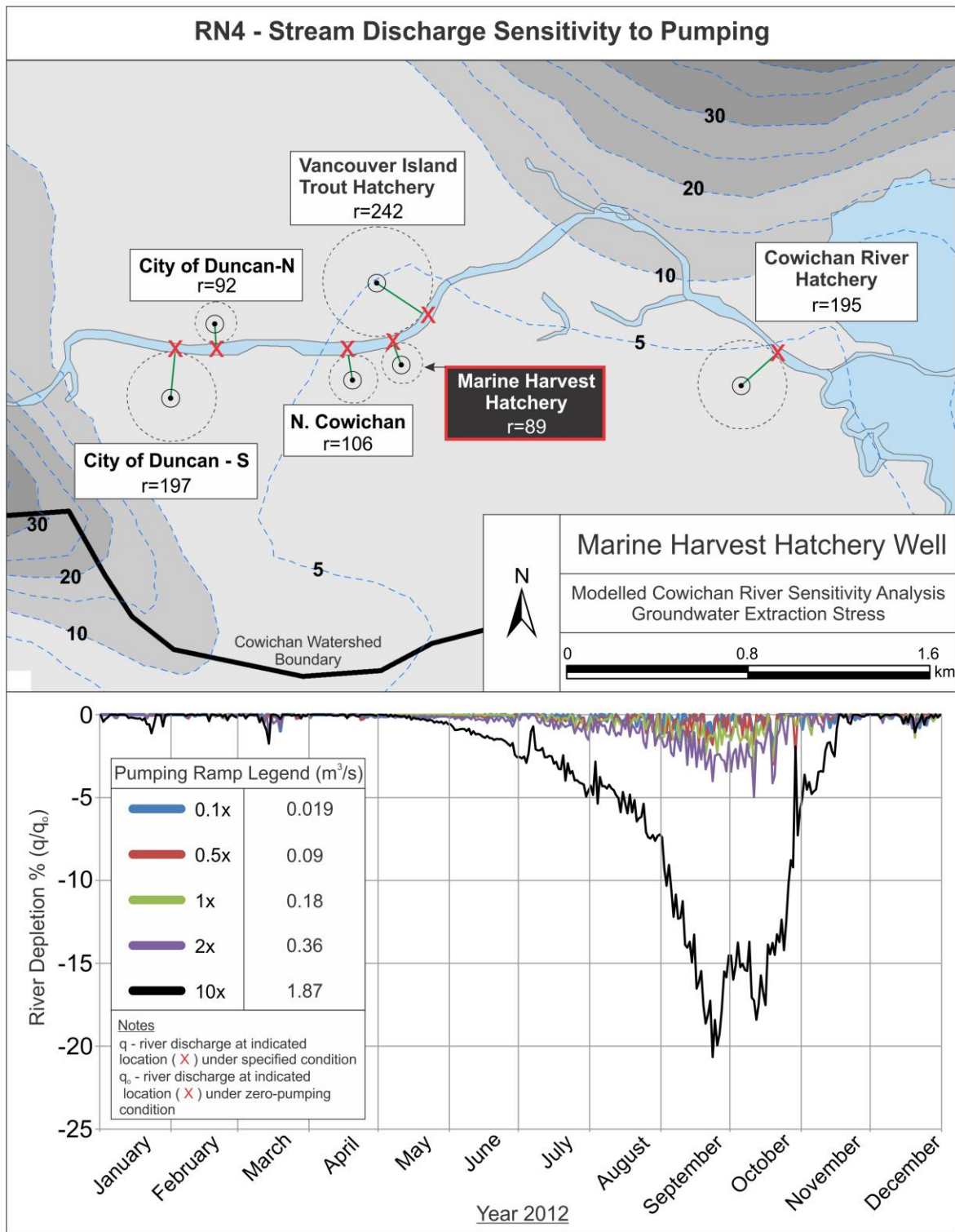
Figure A1.4. Cowichan River depletion assessment - variable pumping rates for the Marine Harvest Hatchery well.
