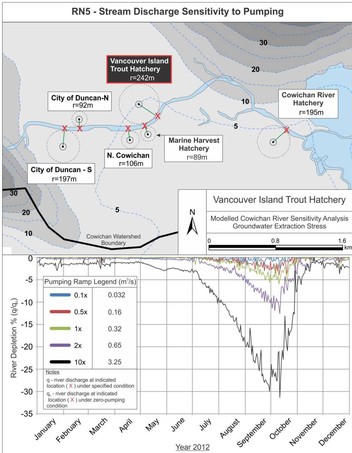
Figure A1.5. Cowichan River depletion assessment - variable pumping rates for the Vancouver Island Trout Hatchery well.
