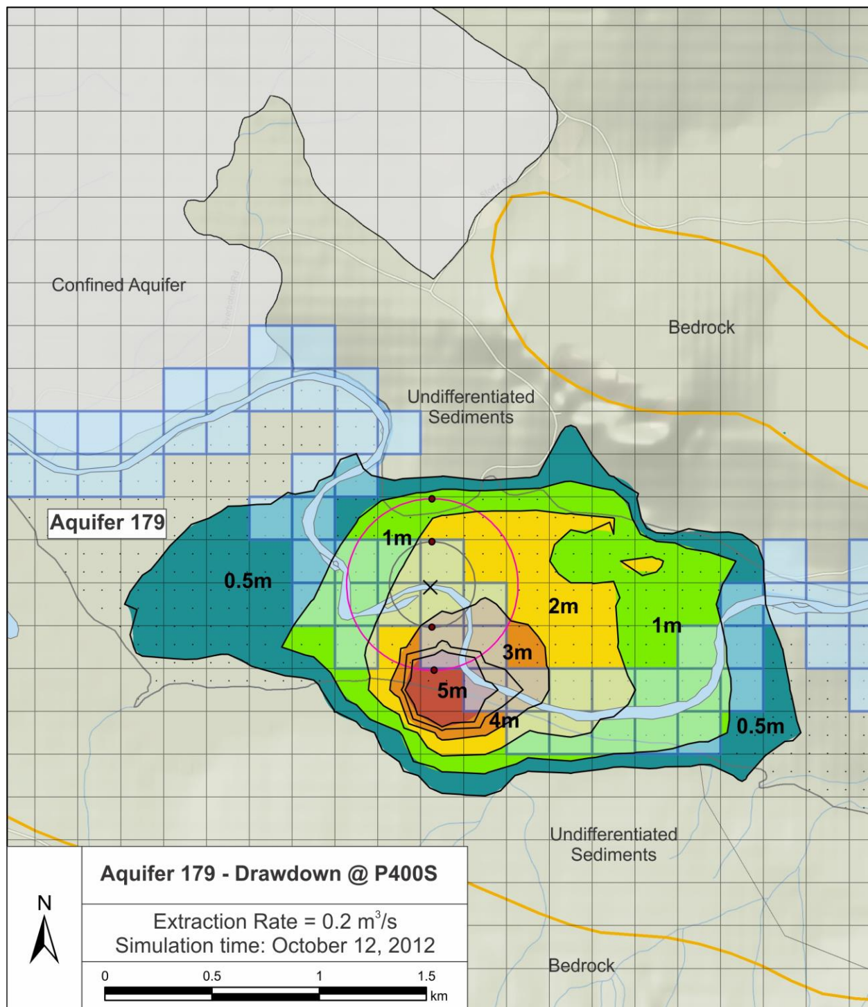
Figure A2.3. Drawdown during distance - sensitivity test. Pumping occurring at P400S location ( 0.2 \text{ m}^3/\text{s} ).
