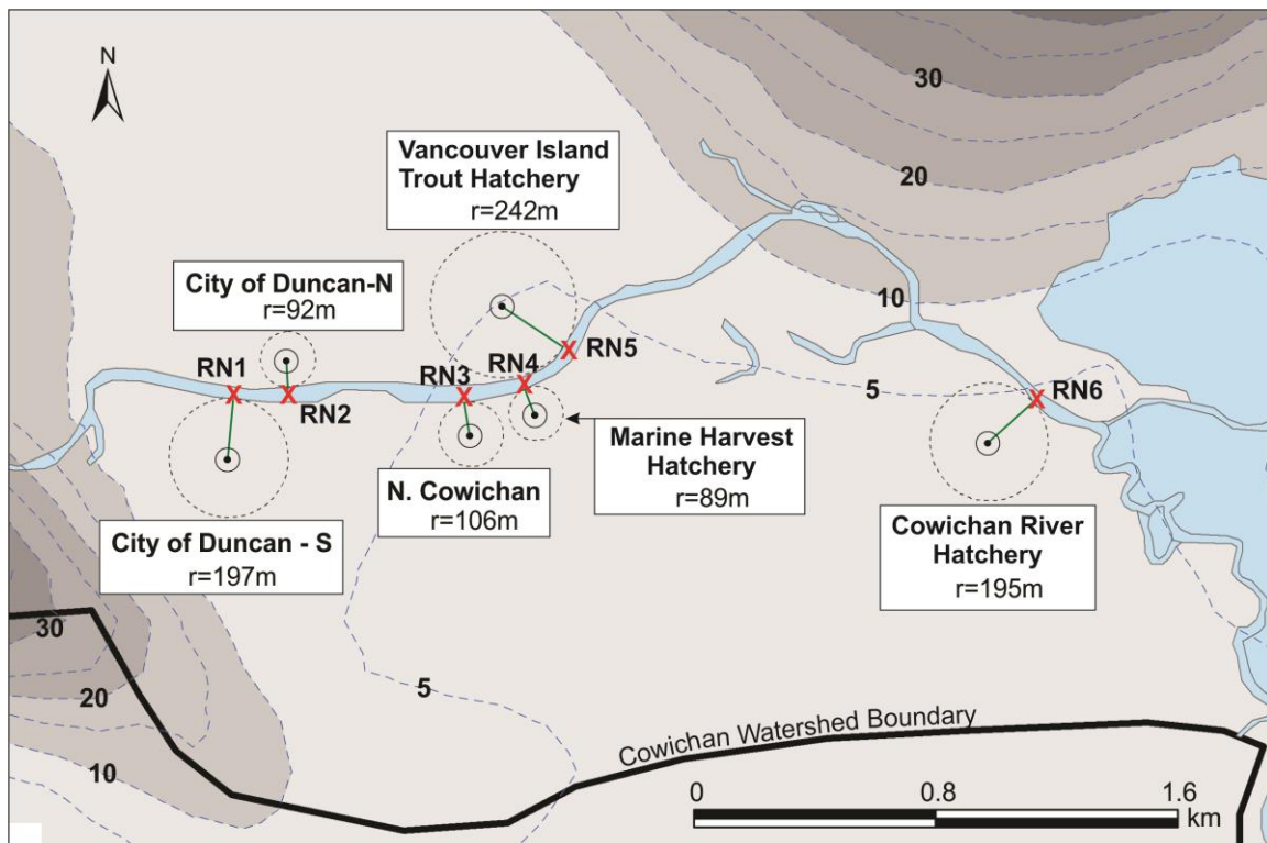
Figure 3.17. Modelled groundwater extraction wells along the Lower Cowichan River. The red Xs represent the closest surface water river node.
