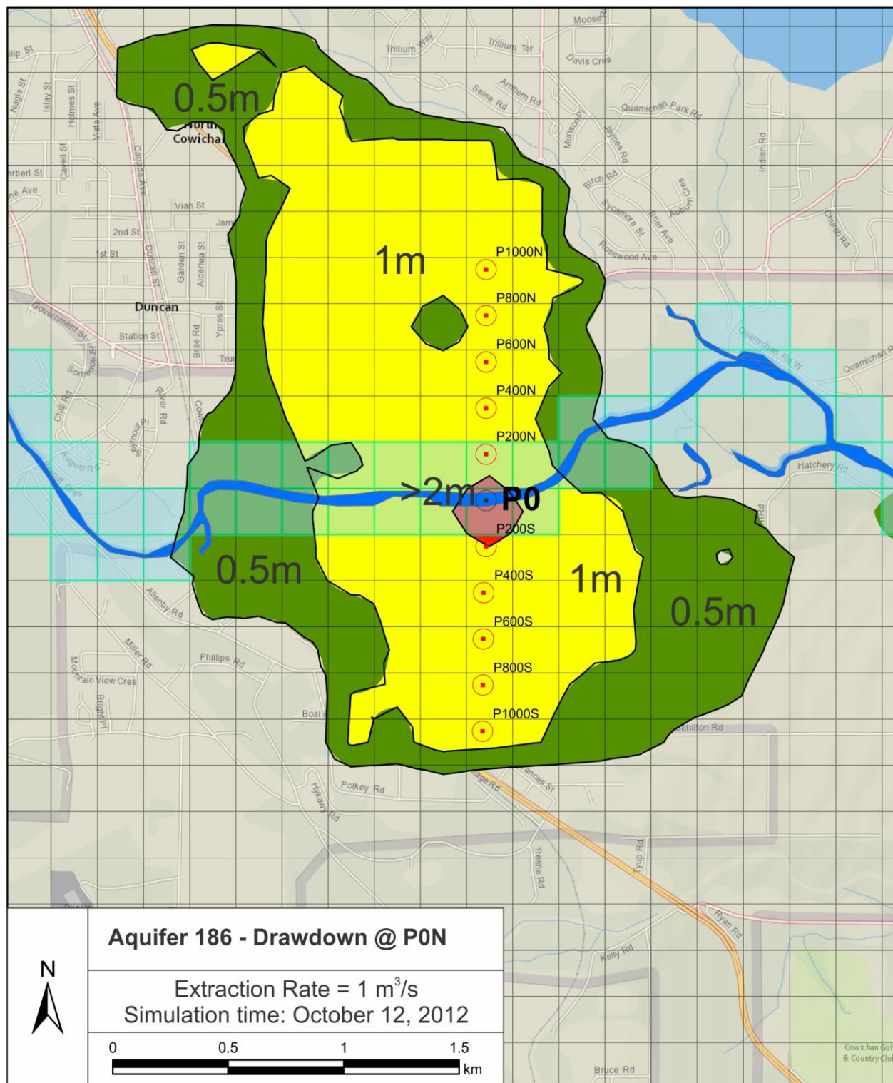
Figure 3.21. Drawdown during distance - sensitivity test. Pumping occurring at P0 location ( 1 \text{ m}^3/\text{s} ).
