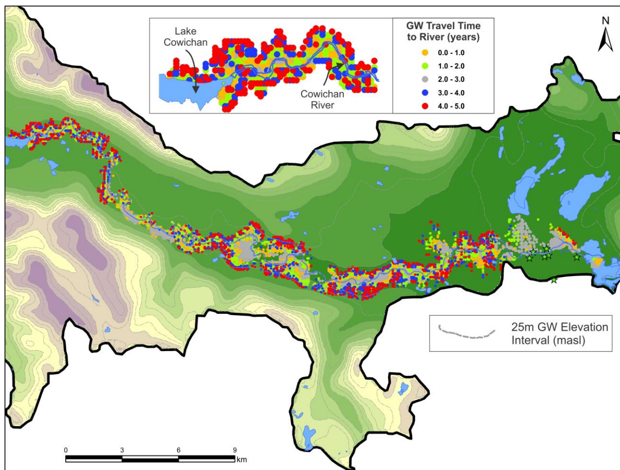
Figure 3.15. 5-year transient “river capture zone analysis” of the Cowichan River.
