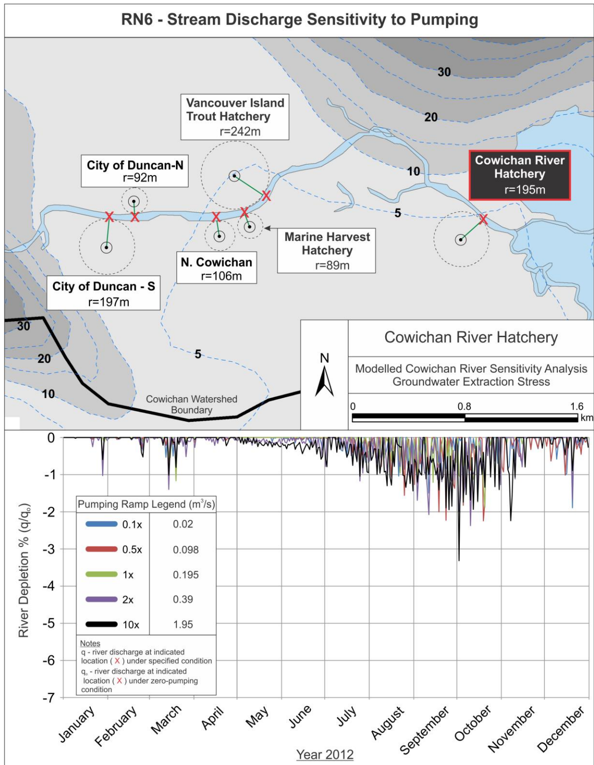
Figure A1.6. Modelled Cowichan River depletion assessment - variable pumping rates for the Cowichan River Hatchery well.
