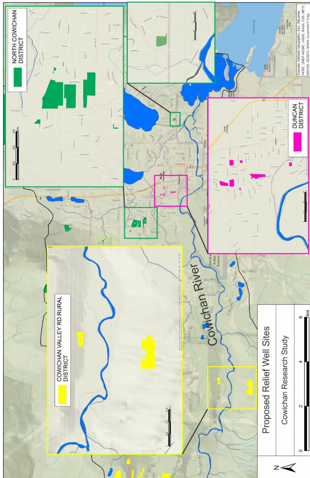
Figure 3.27. Results of the location selection criteria, grouped by location.
