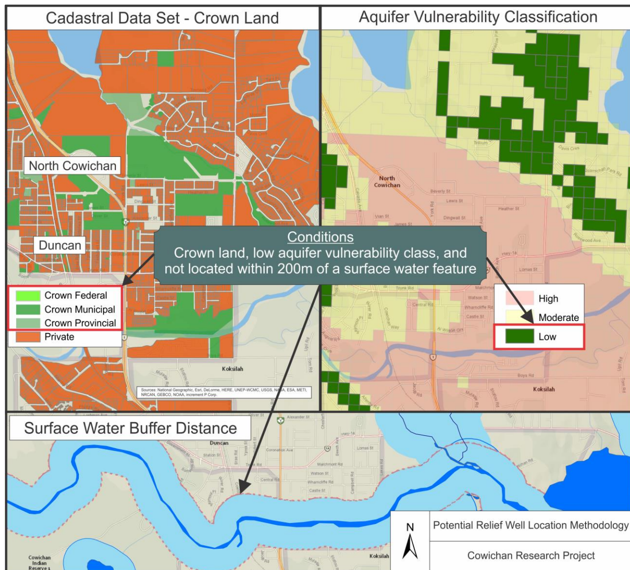
Figure 3.26. Proposed criteria for selecting alternative low flow “relief well” locations.
