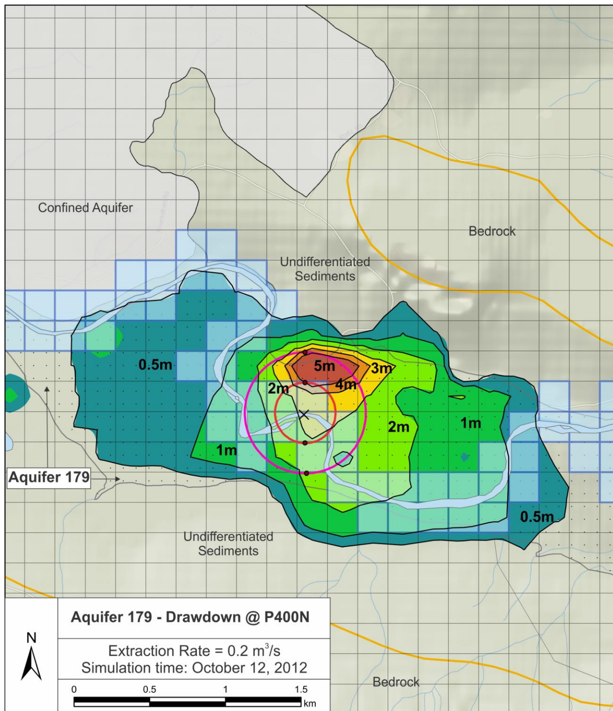
Figure A2.2. Drawdown during distance - sensitivity test. Pumping occurring at P400N location ( 0.2 \text{ m}^3/\text{s} ).
