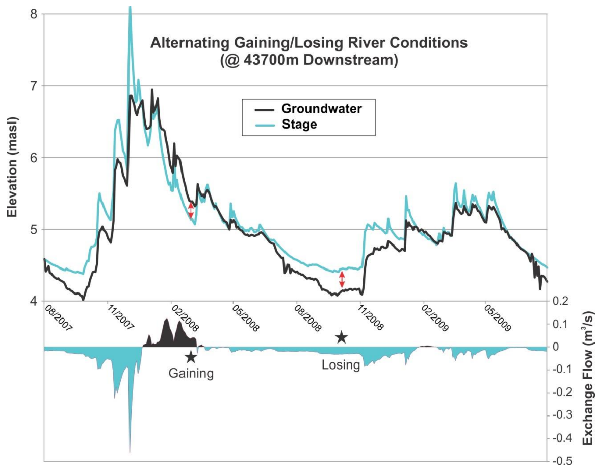
Figure 3.9. Relationship of stage, groundwater levels, and GW-SW exchange.
