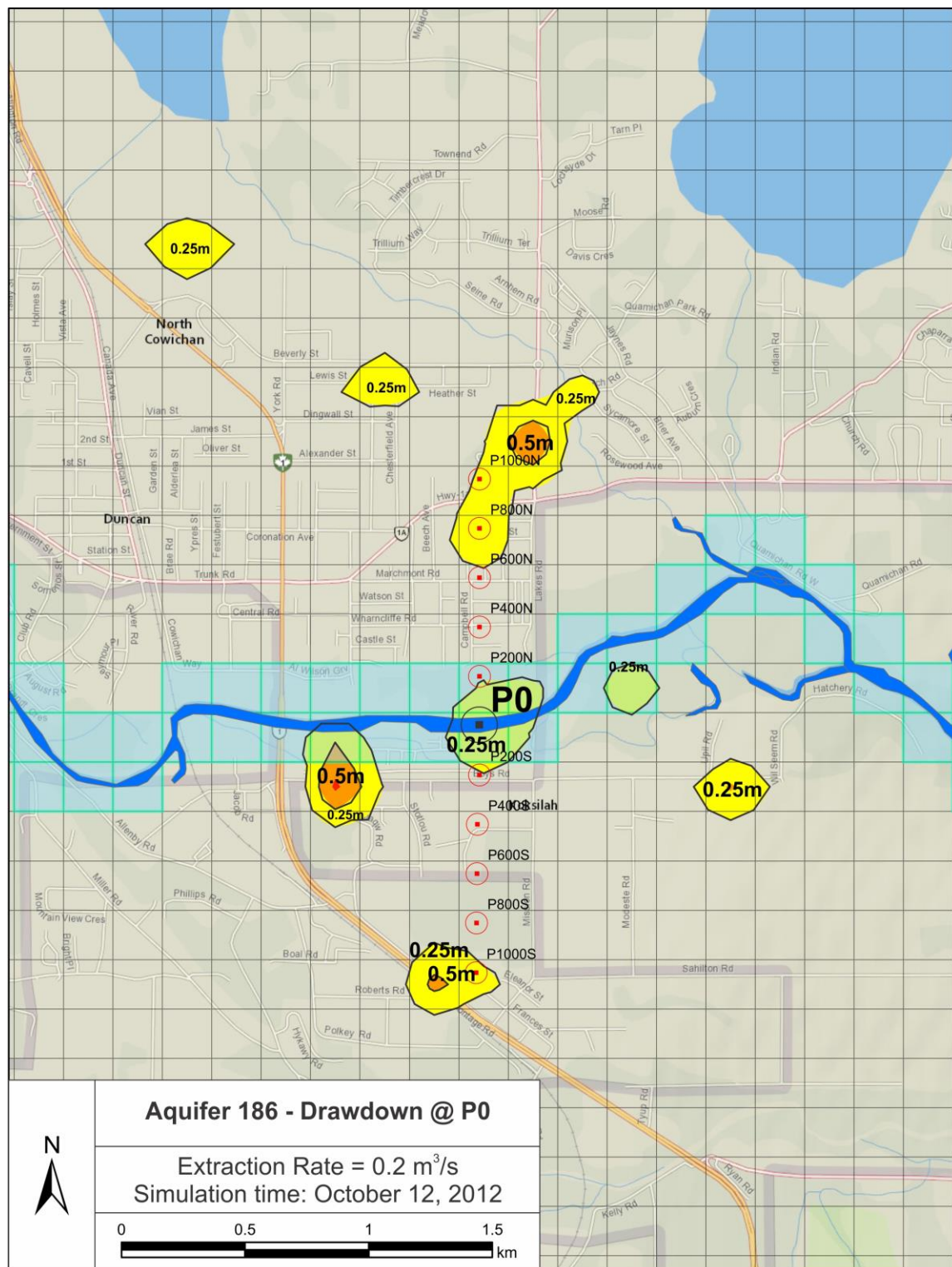
Figure 3.25. Drawdown during distance - sensitivity test. Pumping occurring at P0 location ( 0.2 \text{ m}^3/\text{s} ).
