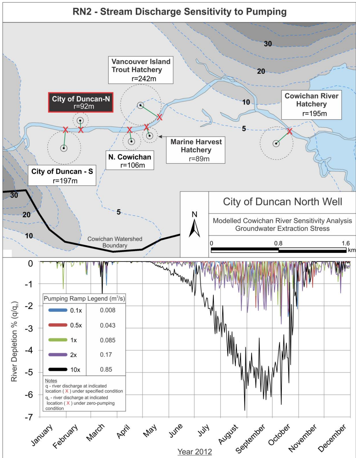
Figure A1.2. Cowichan River depletion assessment - variable pumping rates for the City of Duncan N well.
