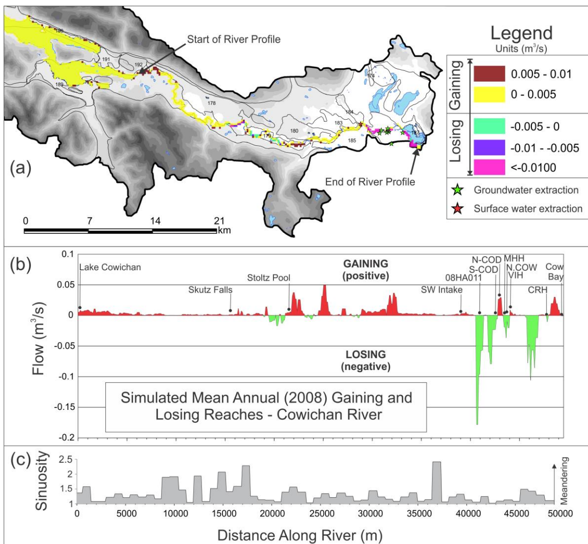
Figure 3.6. Simulated annual (2008) gaining and losing Sections of river in (a) plan view, and (b) profile view (c) sinuosity of the Cowichan River.
