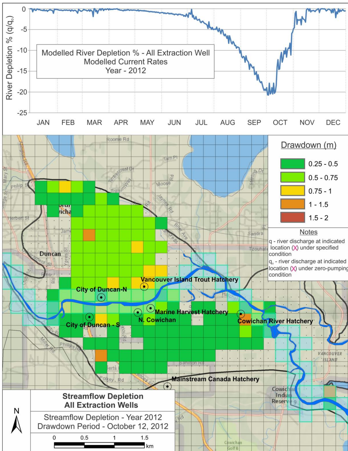
Figure 3.19. Drawdown assessment for all extraction wells pumped at their current rates during the low-flow period in 2012.
