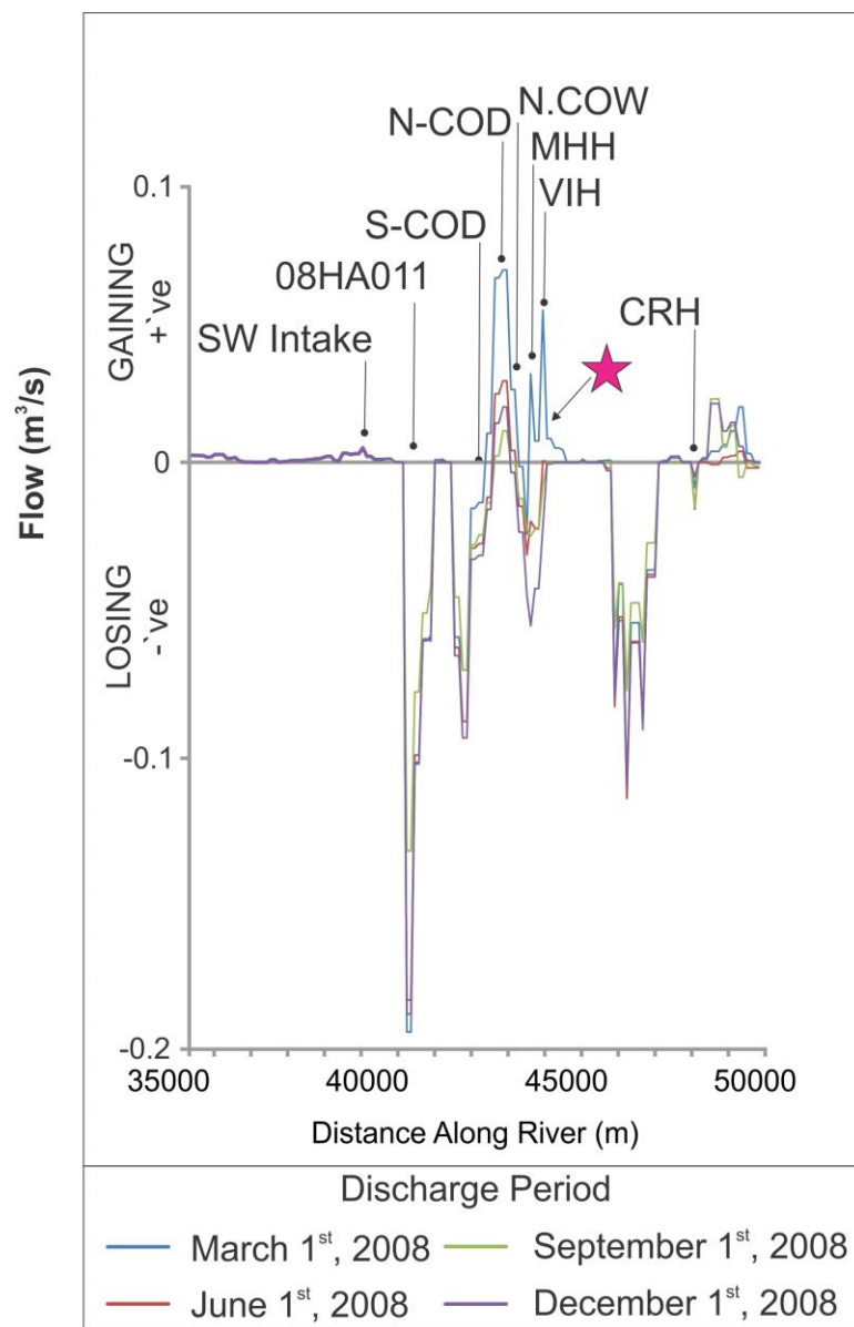
Figure 3.8. Seasonal variations in GW-SW interactions for the lower reaches of the Cowichan River. Note, the red star shows the location of seasonal variation of exchange conditions (see Figure 3.9) (from Foster and Allen 2015).
