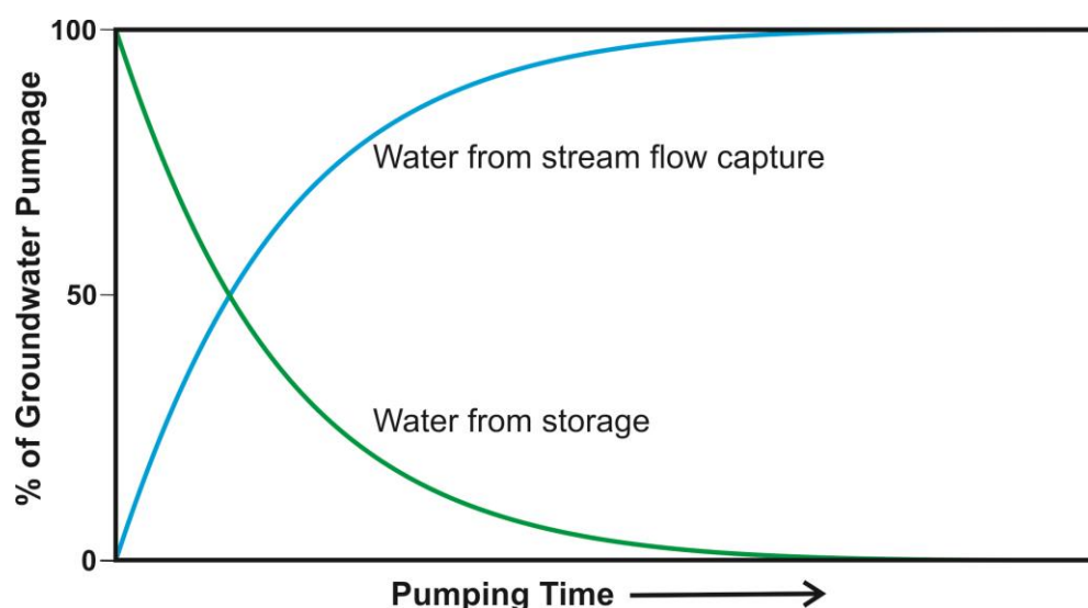
Figure 3.16. Hypothetical situation where the principal source of water to a well can change with time from groundwater storage to capture of streamflow (from Alley et al. 1999).
