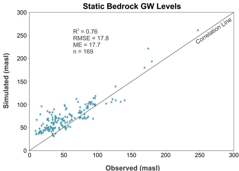
Figure 3.2. Simulated mean annual (2007) bedrock GW elevations verses observed static GW elevations in bedrock from the BC WELLS database.
