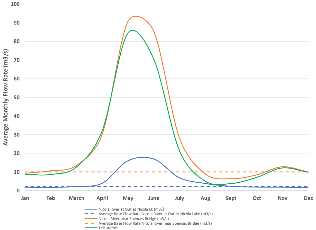
Figure 14: Mean monthly and annual average flow rates in Nicola River
