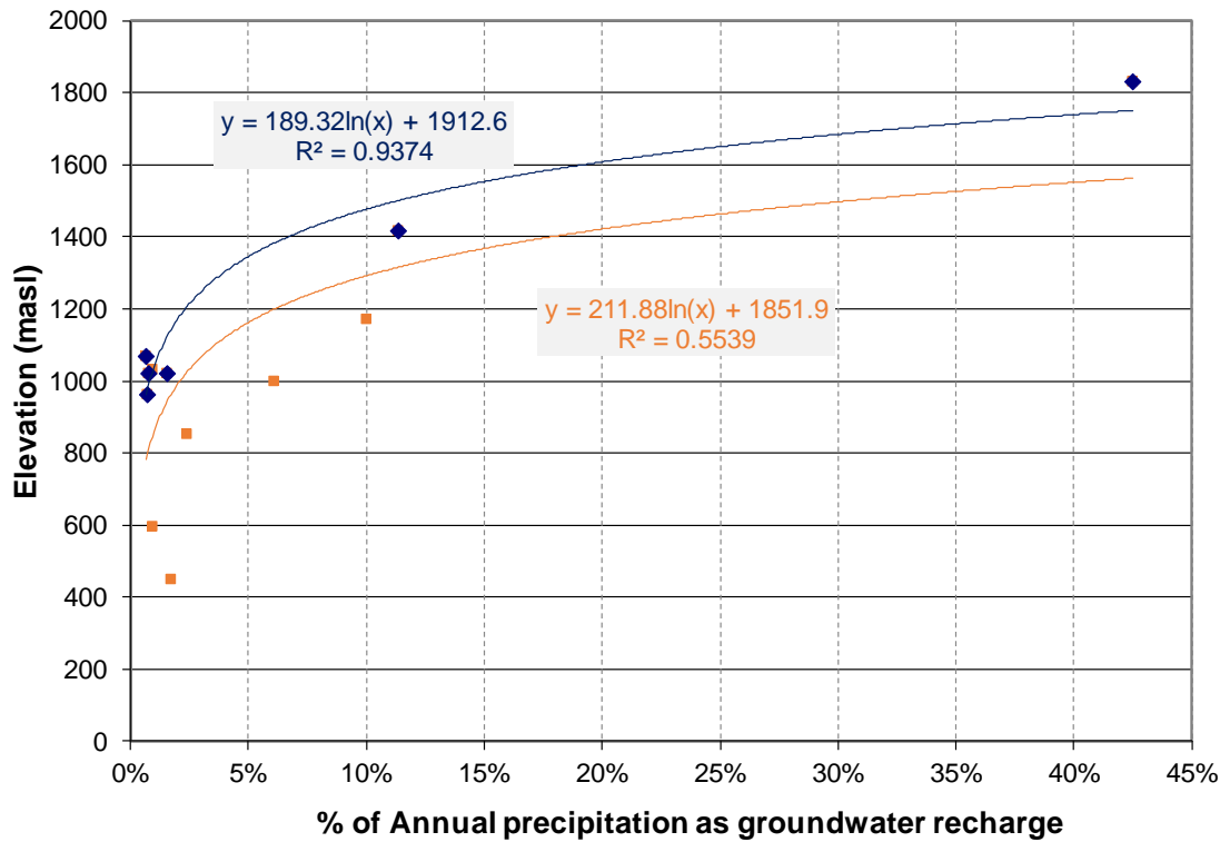
Figure 9: Percent of annual precipitation as groundwater recharge vs elevation
