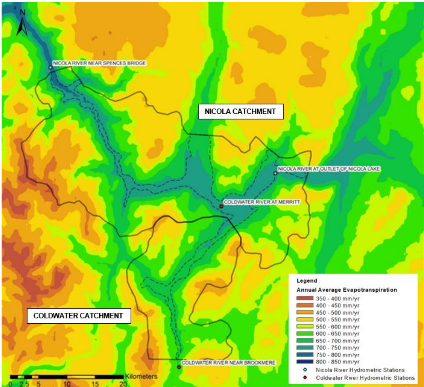
Figure 3: Map of annual average potential evapotranspiration by elevation (mm/year)
