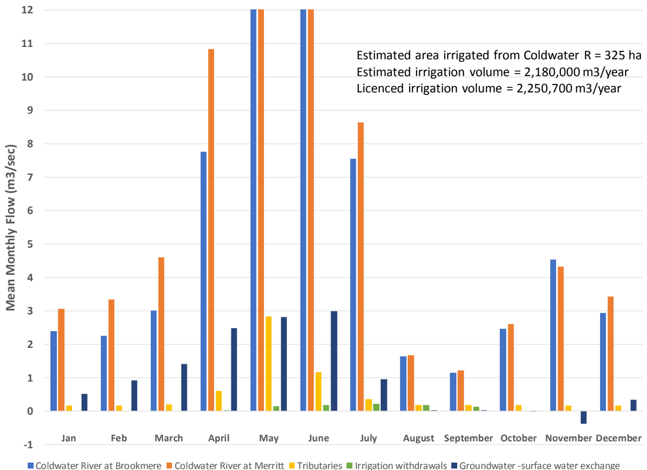
Figure 17: Coldwater River hydrograph
