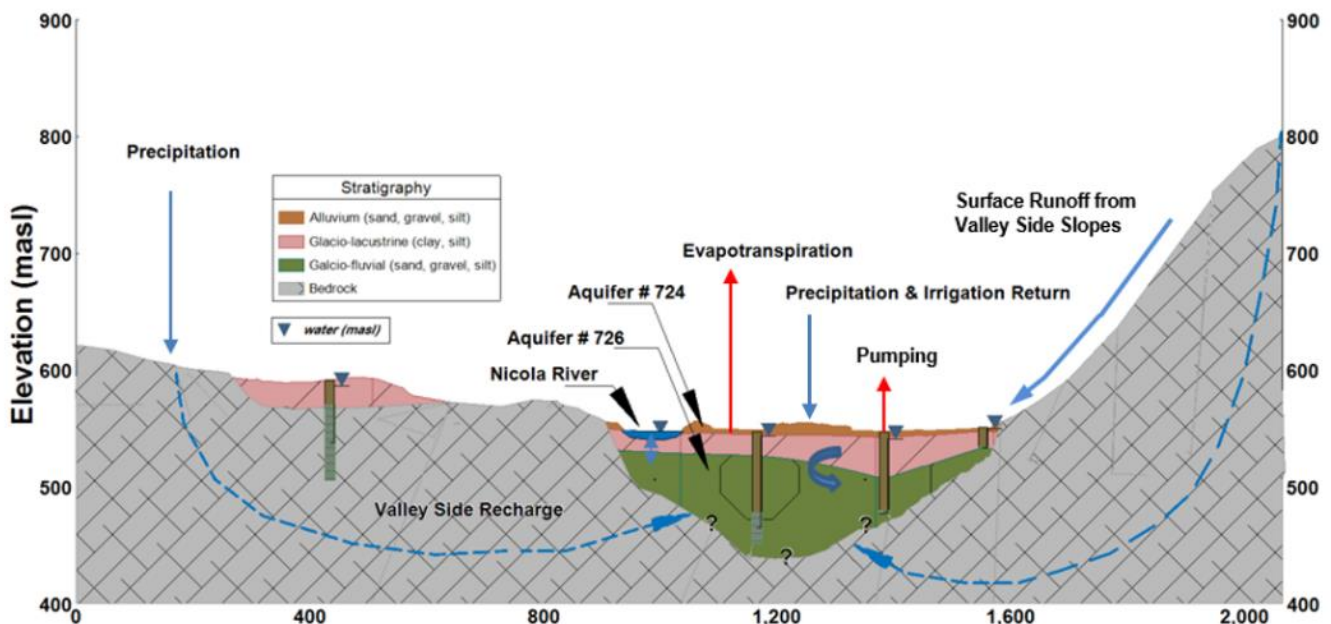
Figure 7: Conceptual cross-section illustration of recharge (blue arrows) to and discharge (red arrows) from valley sediments
