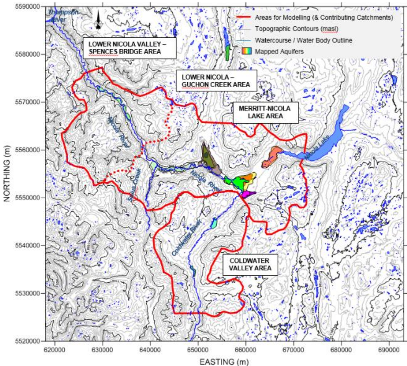
Figure 1: Area Plan illustrating model study areas and mapped aquifers (Golder 2018b)
