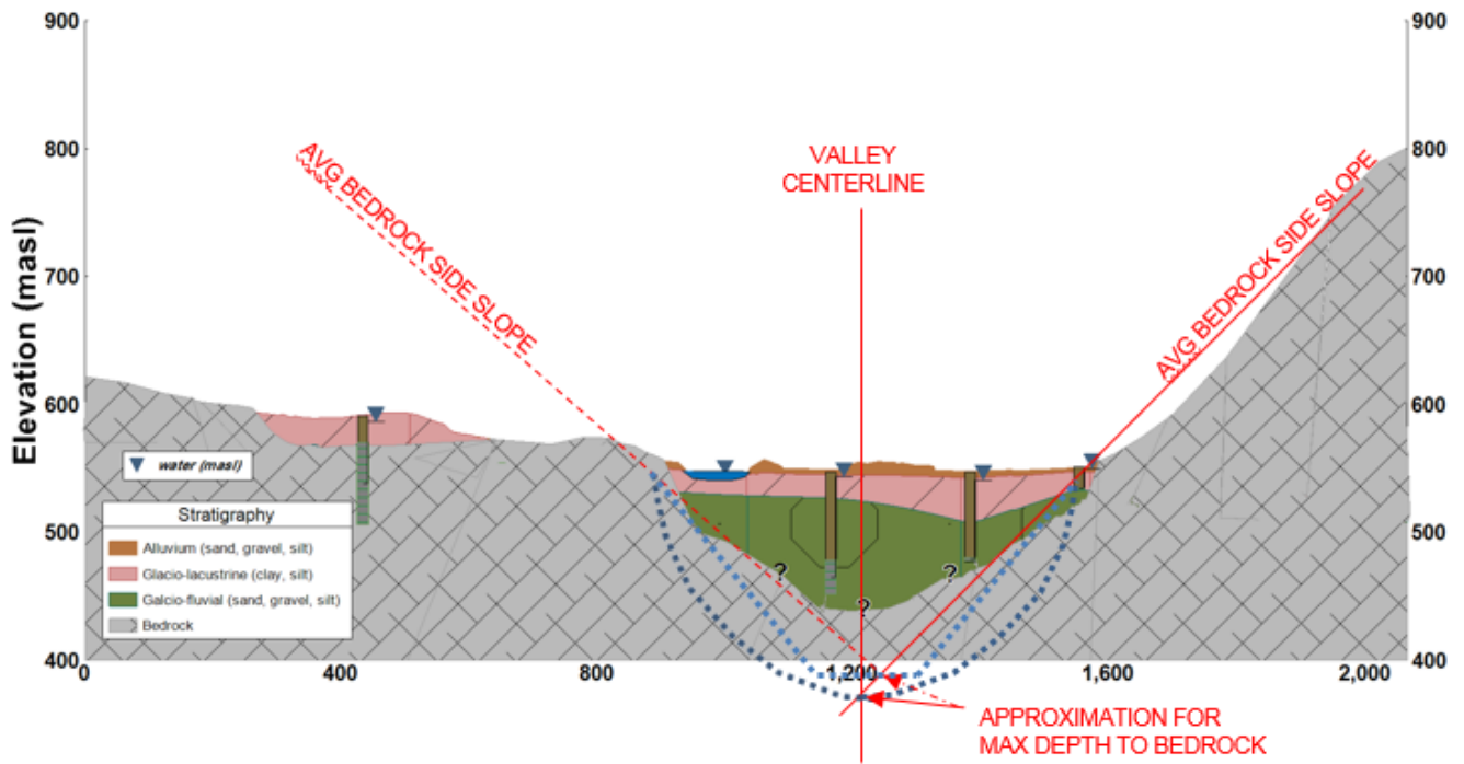
Figure 6: Geologic cross-section (Golder 2016) and method to extrapolate bedrock surface
