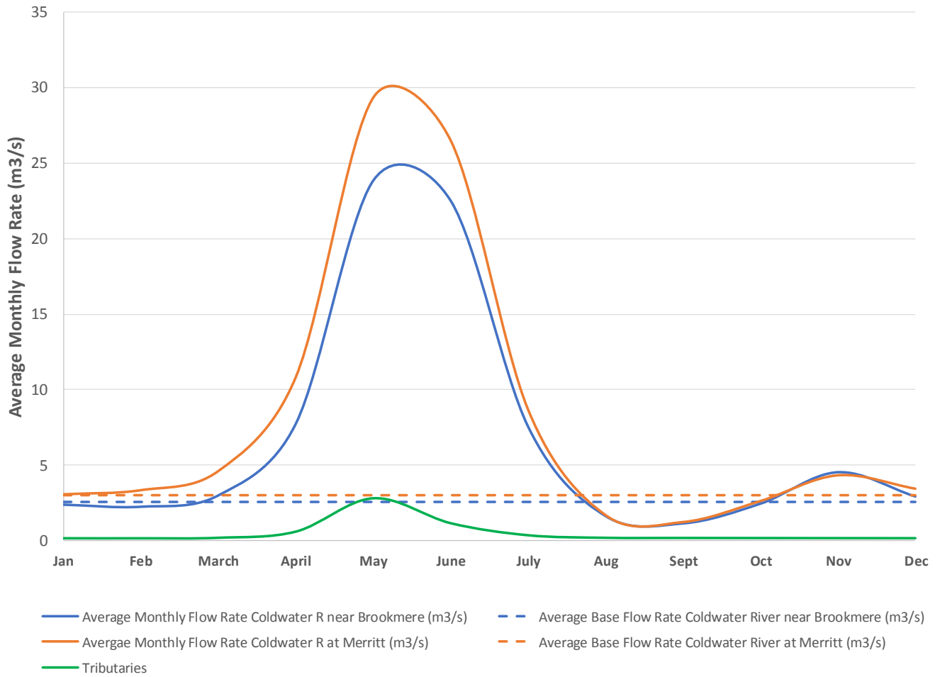
Figure 13: Mean monthly and annual average flow rates in Coldwater River
