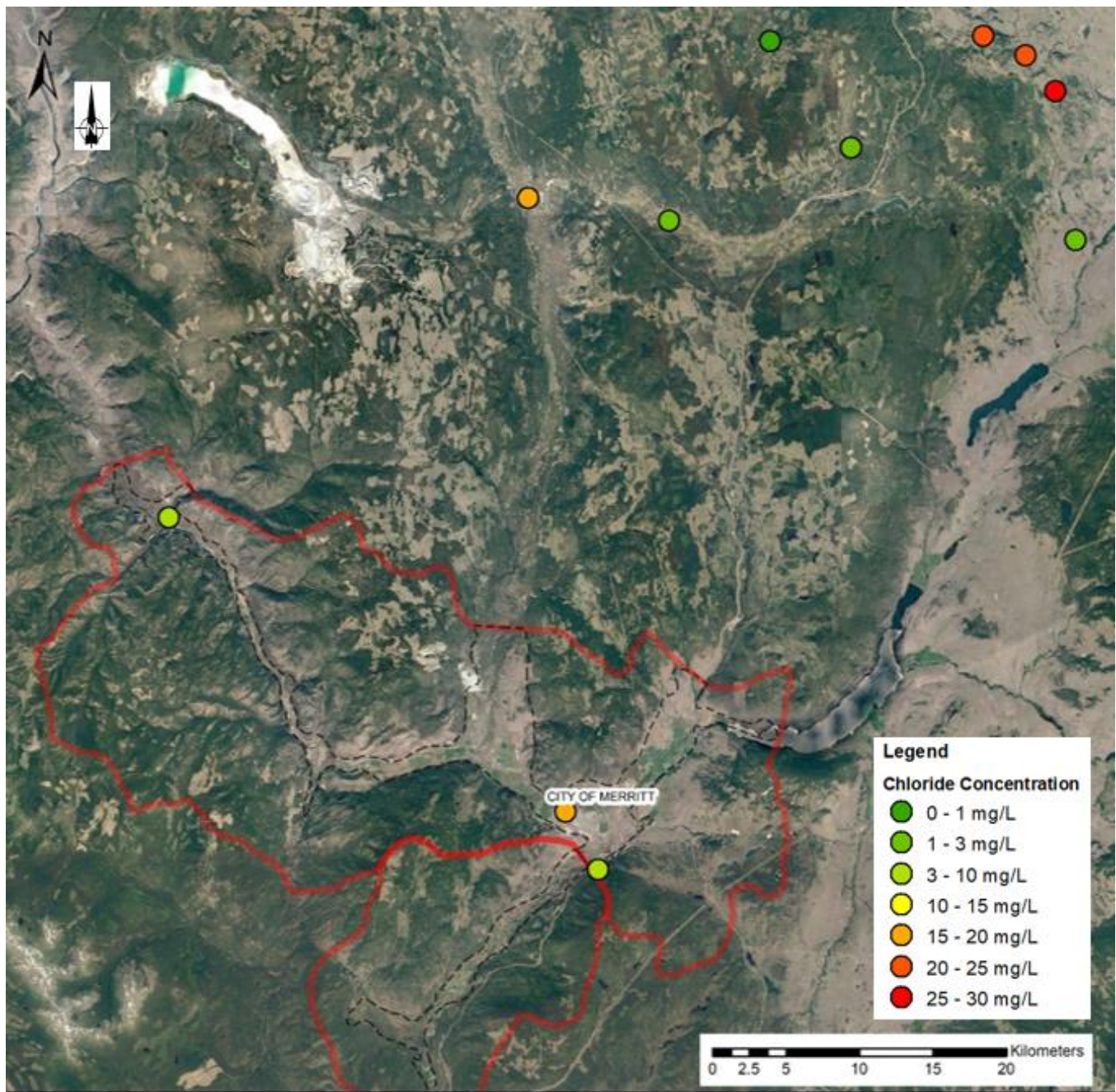
Figure 8: Groundwater chloride sampling locations in the Kamloops-Merritt area
