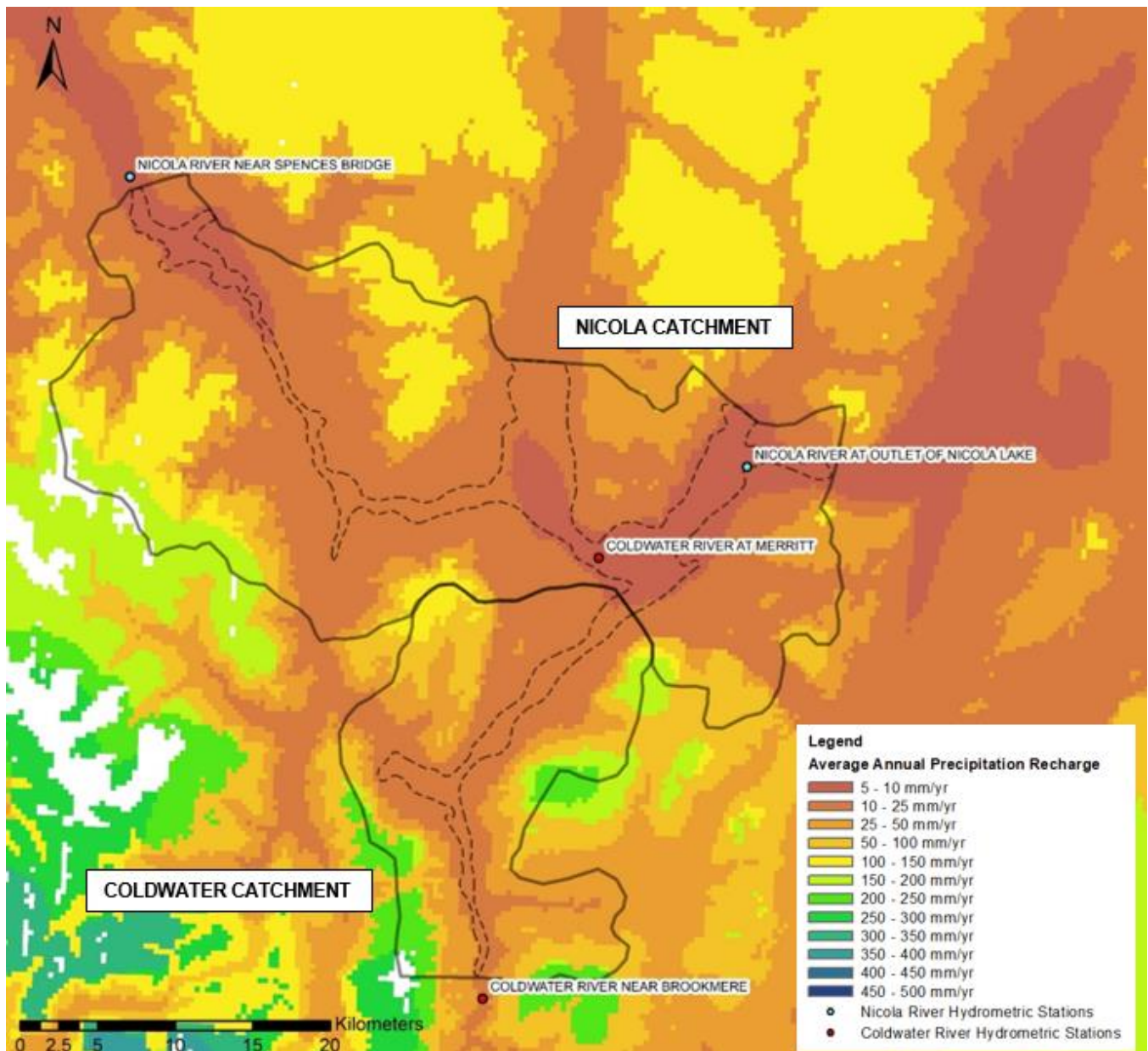
Figure 10: Estimated groundwater recharge from precipitation by elevation in the study area
