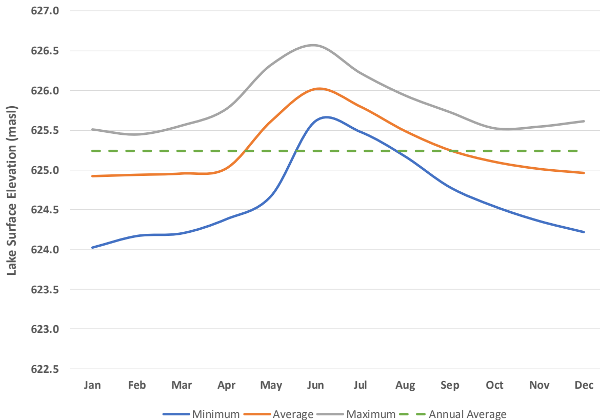
Figure 15: Average monthly surface elevation of Nicola Lake (1933 – 2015)
