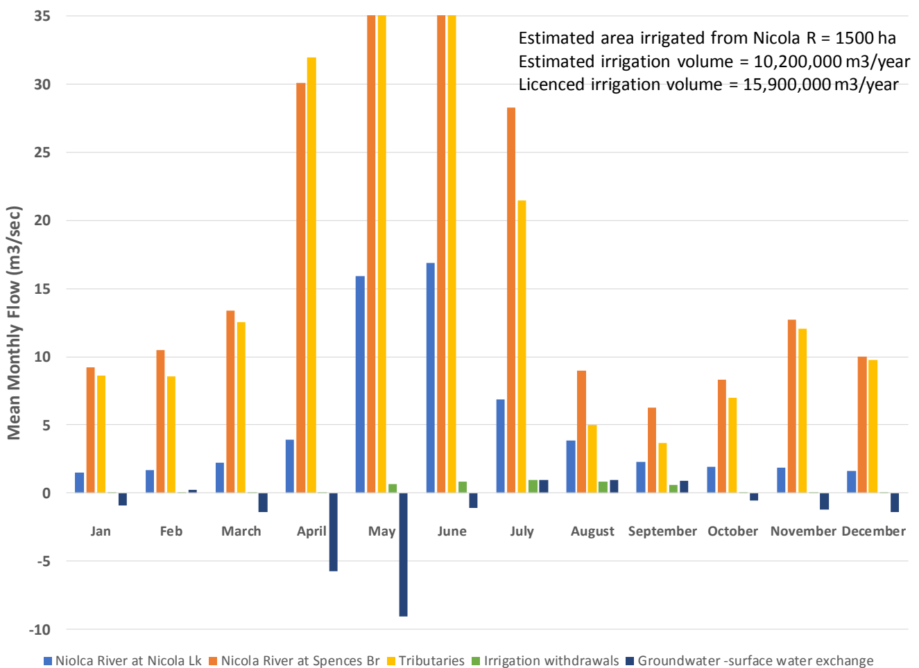
Figure 16: Nicola River Hydrograph
