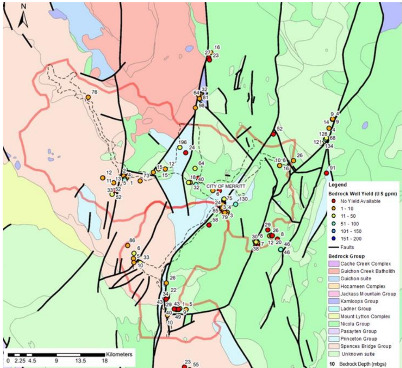
Figure 5: Map of bedrock geology, bedrock water well yields (US gpm) and depth to bedrock below surface (m)
