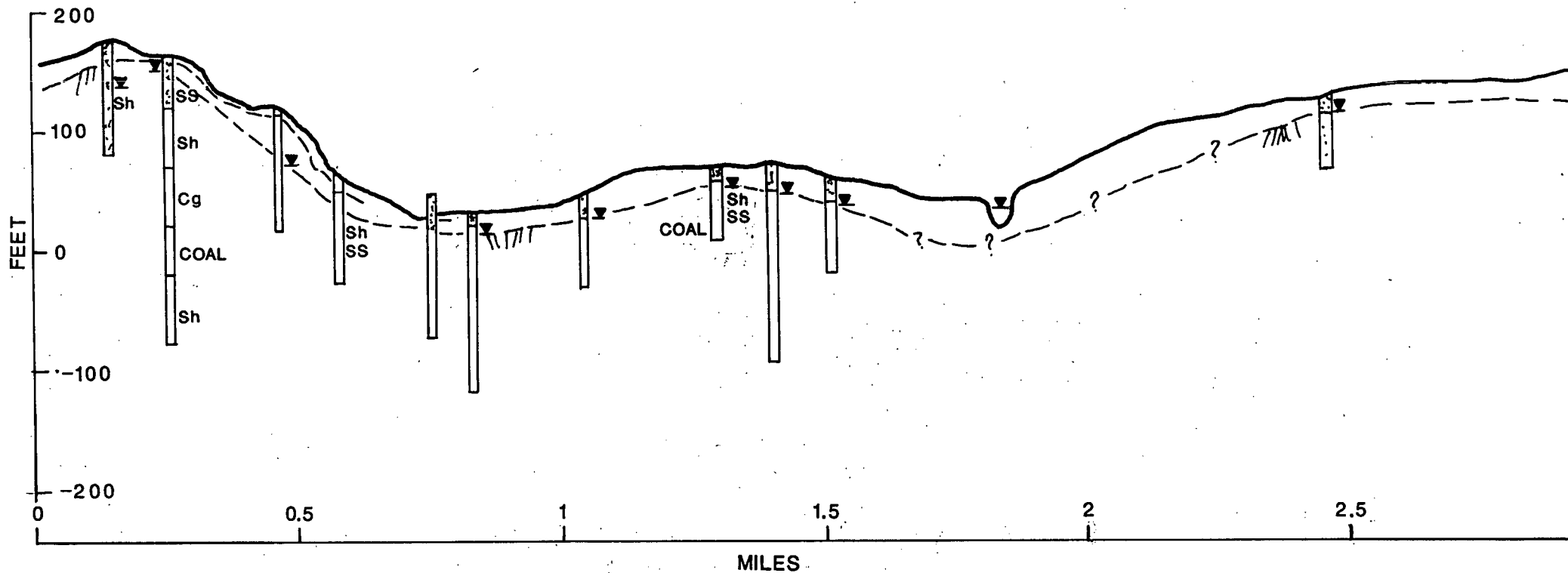
FIGURE 7 CROSS SECTION 5-5
