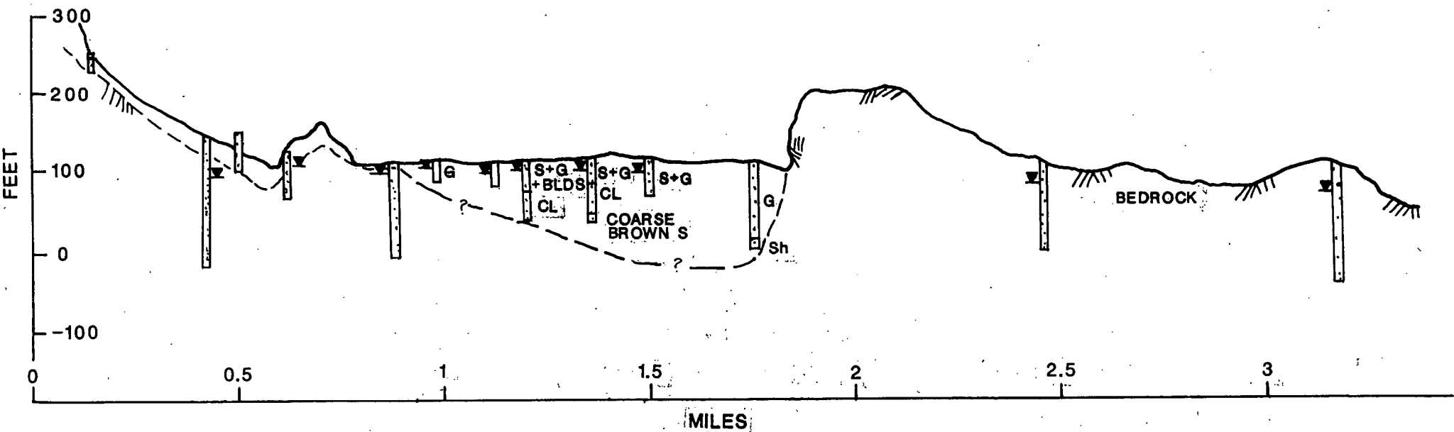
FIGURE 9 CROSS SECTION 8-8
