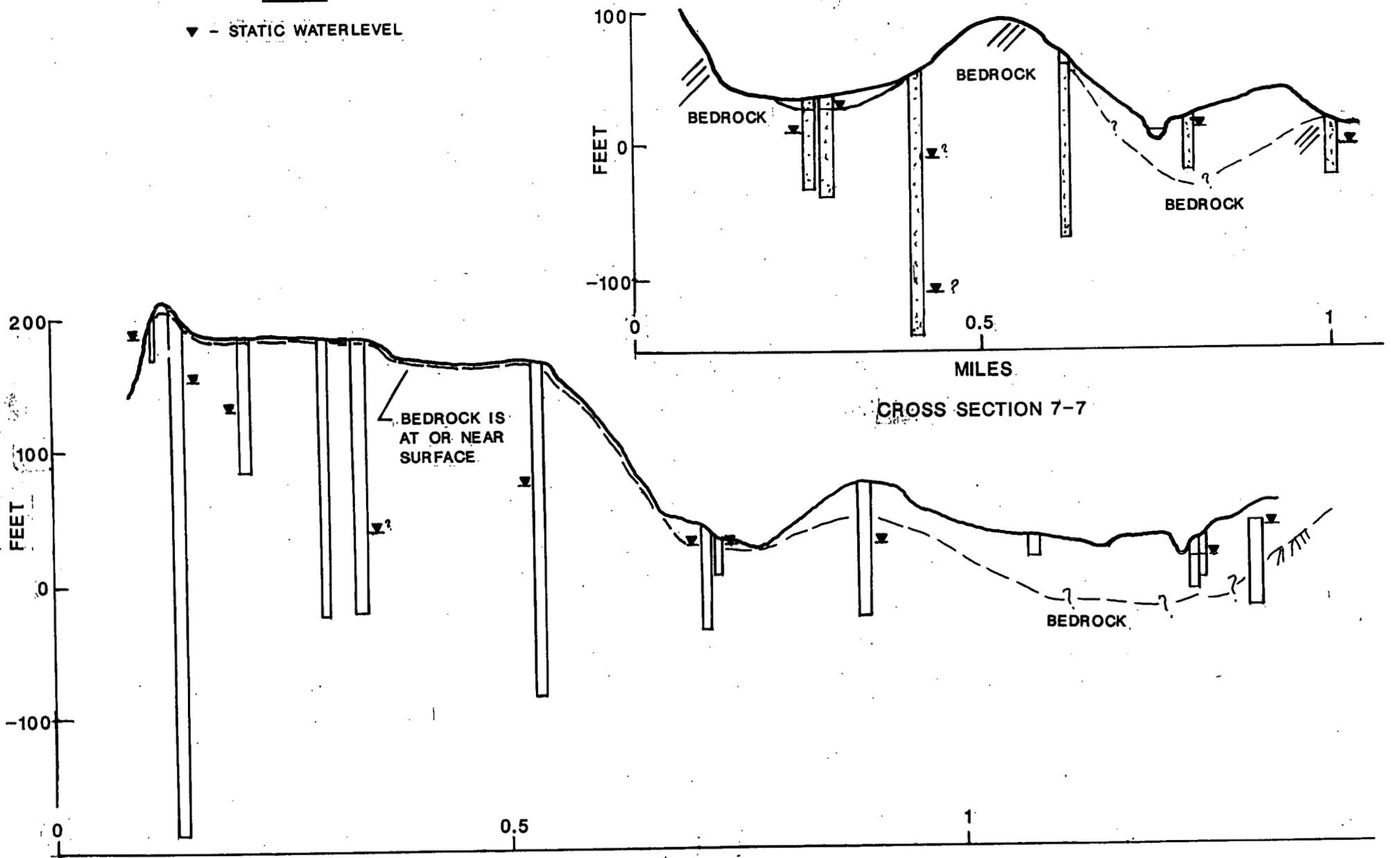
FIGURE 18 CROSS SECTION 6-6 NANAIMO RIVER BASIN GROUNDWATER RESOURCE EVALUATION (AUG. 1991)
