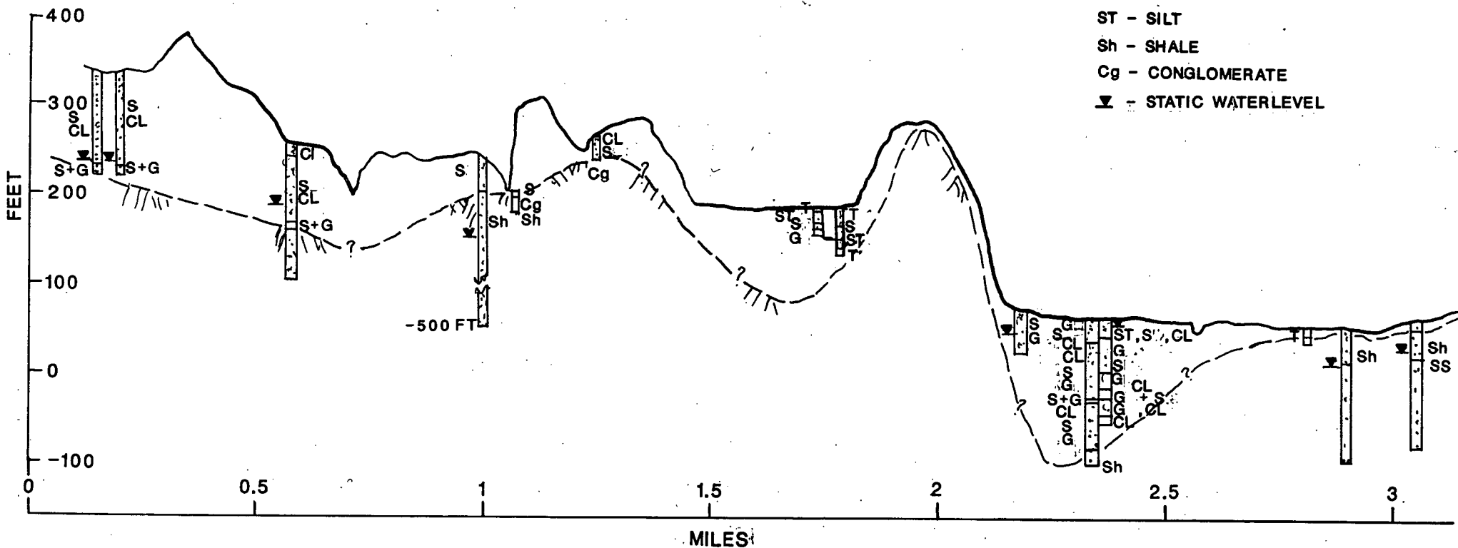
FIGURE 6 CROSS SECTION 4-4 NANAIMO RIVER BASIN GROUNDWATER RESOURCE EVALUATION (AUG. 1991)
