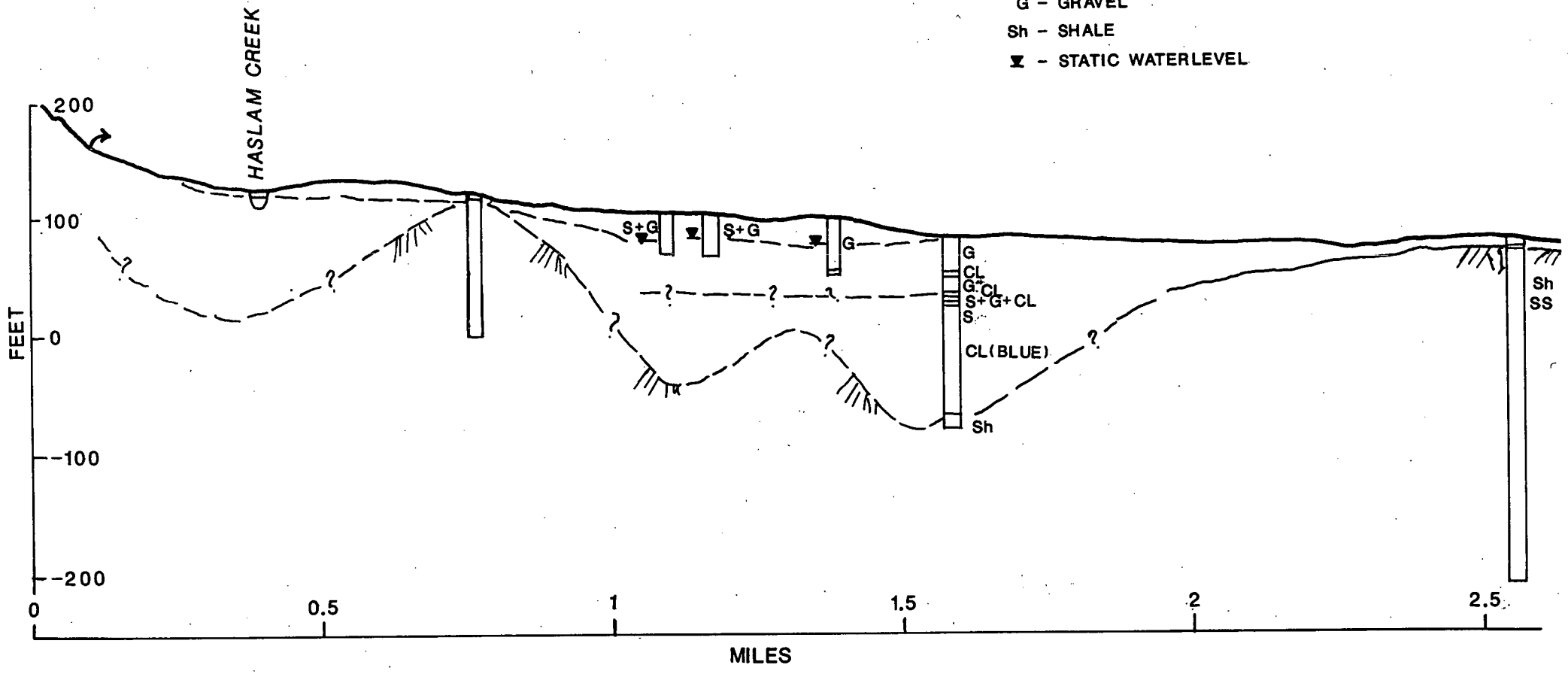
FIGURE 5 CROSS SECTION 3-3 NANAIMO RIVER BASIN GROUNDWATER RESOURCE EVALUATION (AUG. 1991)
