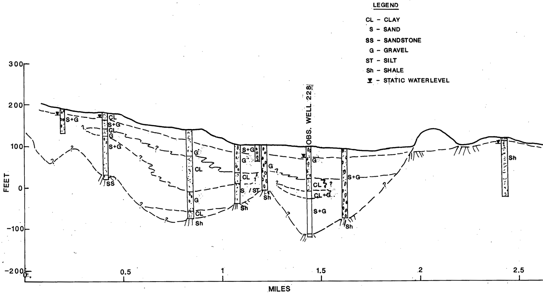
FIGURE 4 CROSS SECTION 2-2
