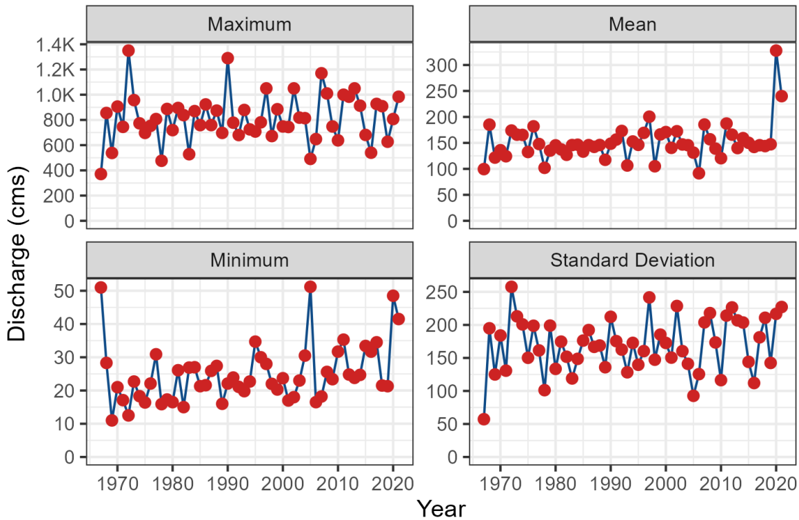
Figure 2.3: Summary discharge statistics (annual maximum, minimum, mean and standard deviation) for Parsnip River at hydrometric station #07EE007.
