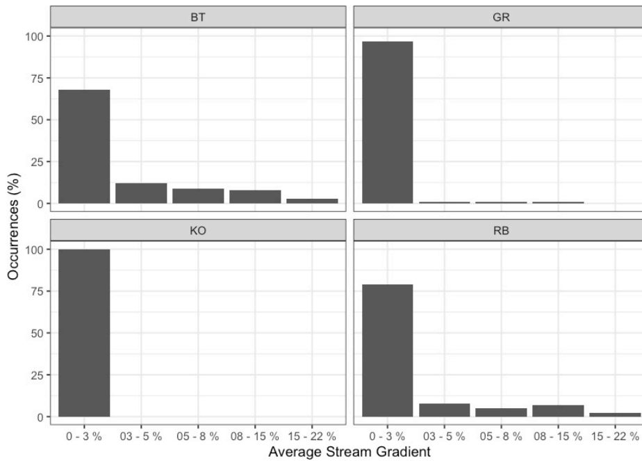
Figure 2.4: Summary of historic salmonid observations vs. stream gradient category for the Parsnip River watershed group.
