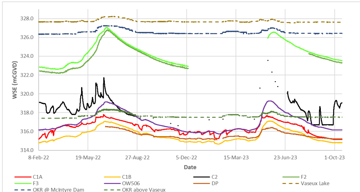
Figure 12: Groundwater level data across the fan. Vaseux Lake, OKR at McIntyre Dam and OKR above Vaseux Creek are included for reference.
