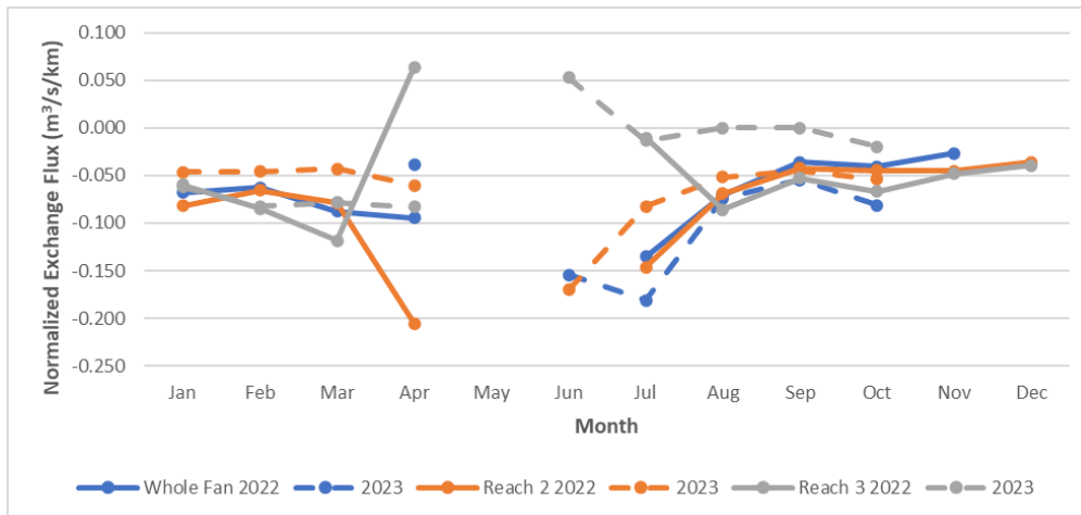
Figure 23: Inter-annual comparison of normalized exchange flux ( m^3/s/km ).
