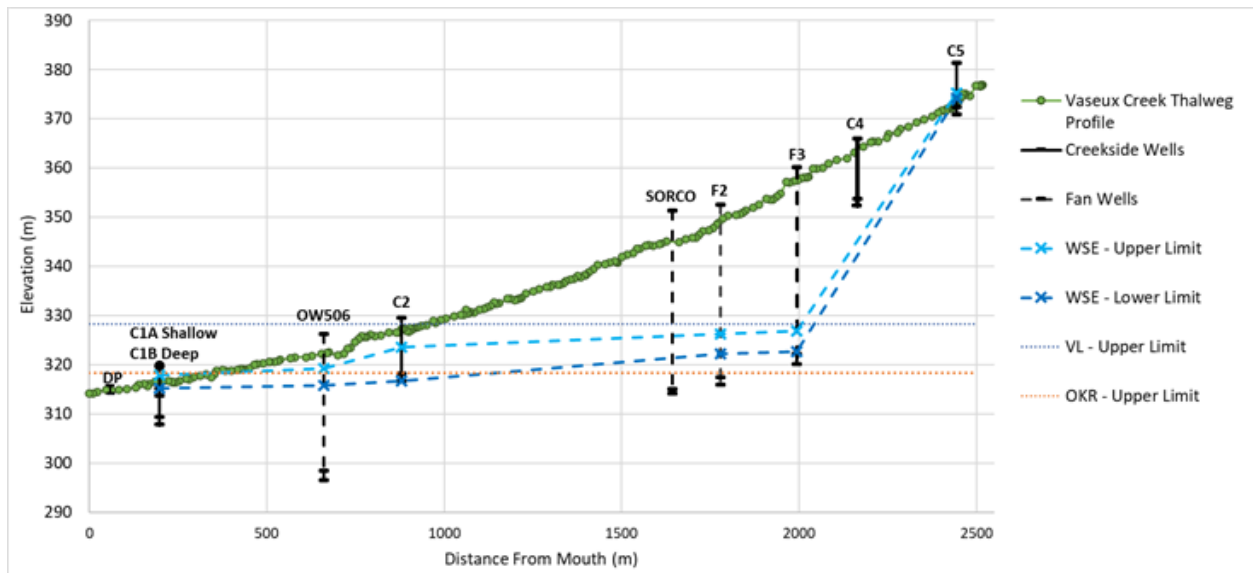
Figure 11: Longitudinal thalweg profile of Vaseux Creek with groundwater wells projected to the profile line. Horizontal markers depict the upper and lower boundaries of well screens. The upper and lower water surface elevation (WSE) limits, Vaseux Lake (VL) and Okanagan River (OKR) high water level are included for hydraulic context (Montgomery, In Prep.).
