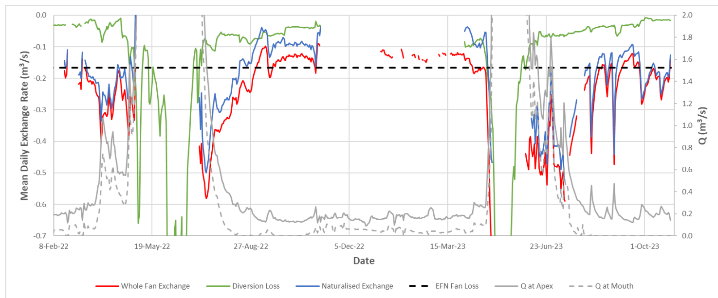
Figure 20: Mean daily exchange rate for the whole fan and the combined diversions. Discharge at the apex and mouth are plotted for reference.
