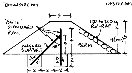
FIGURE 4.4 Details of rail and concrete debris-straining structure.
