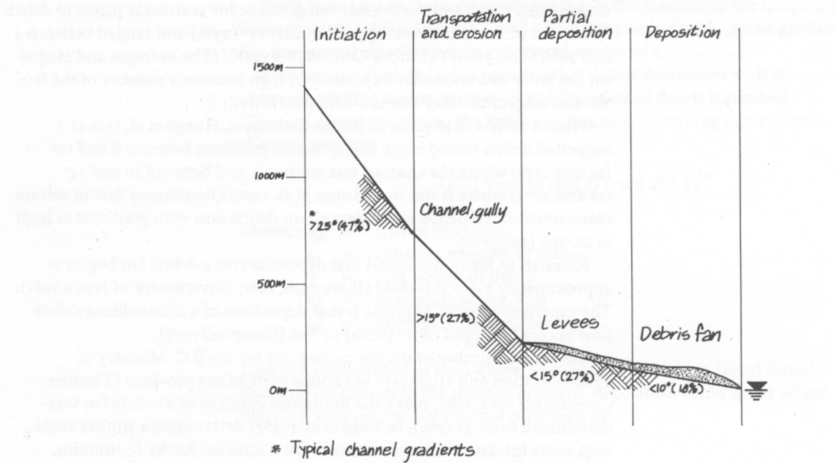
FIGURE 2 Zones of channellized debris flow.
