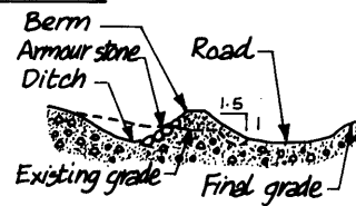
FIGURE 23 Mitigative control structure, small tributary along Riley Mainline.
