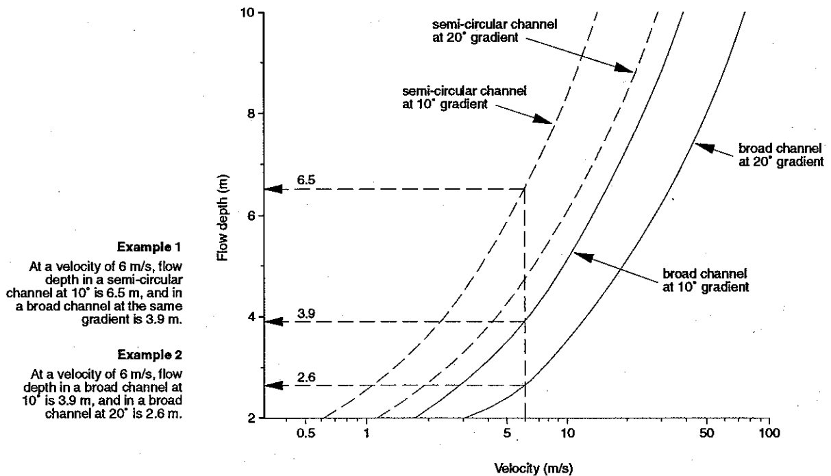
FIGURE 7 Examples of flow height (flow depth) versus velocity, based on Poiseuille Equation.
