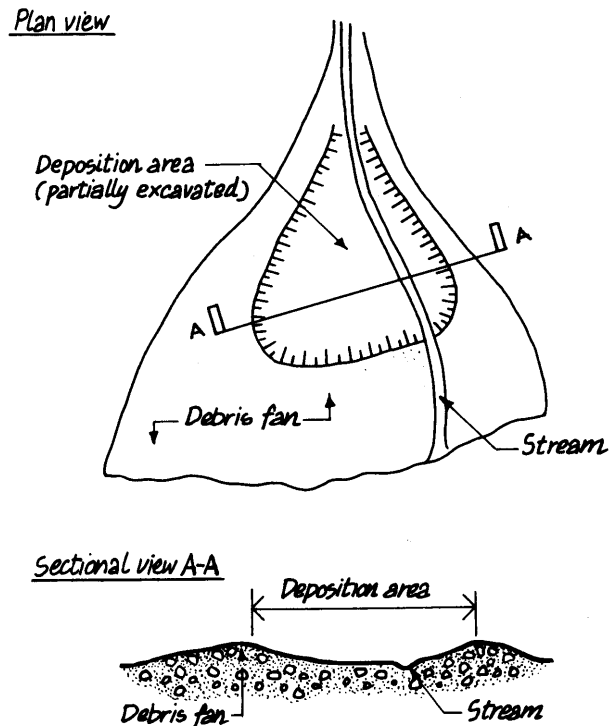
FIGURE 11 Plan and sectional view of an unconfined deposition area.
