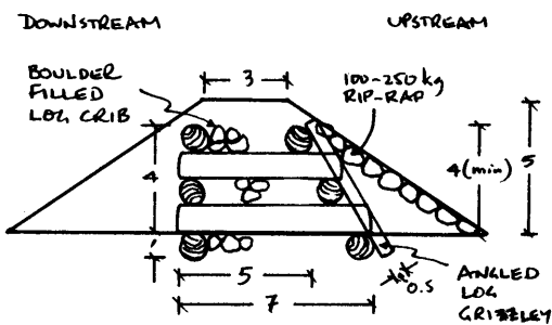
FIGURE 4.3 Details of log crib debris straining structure.
