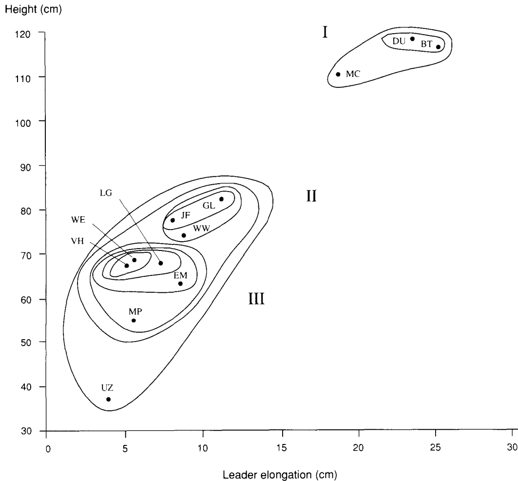
FIGURE 3. Illustration of successive fusion in each step of clustering of the 12 test sites.
